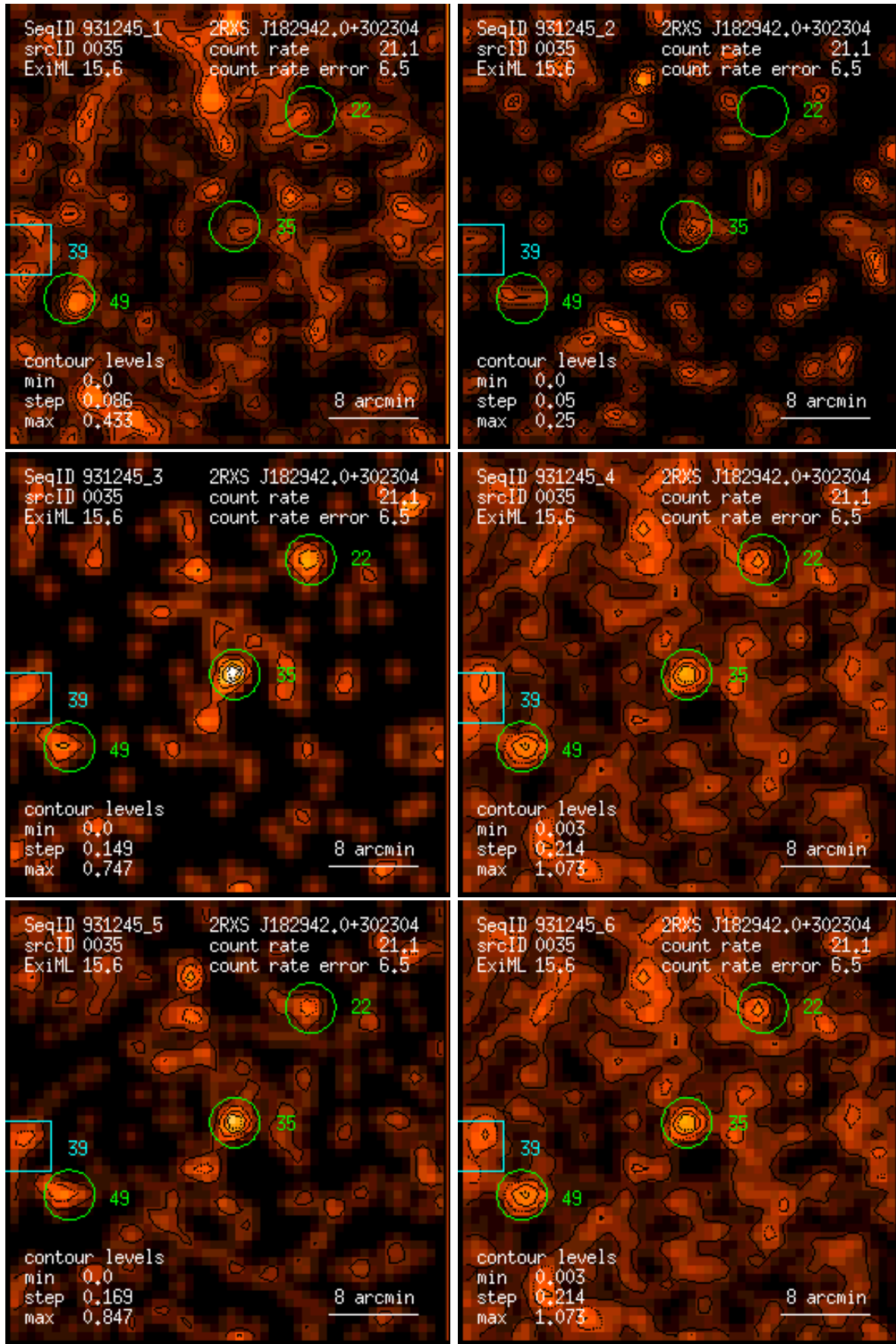
Figure 35: RASS 931245: detection 0035: band rate images, Gaussian filter: (1) PSPC channels 11 – 41, (2) 52 – 90, (3) 91 – 201, (4) 11 – 235, (5) 52 – 201, (6) 11 – 201. Broad band rates in counts/ks. Band rate contour levels in counts/ks/arcmin 2 .
