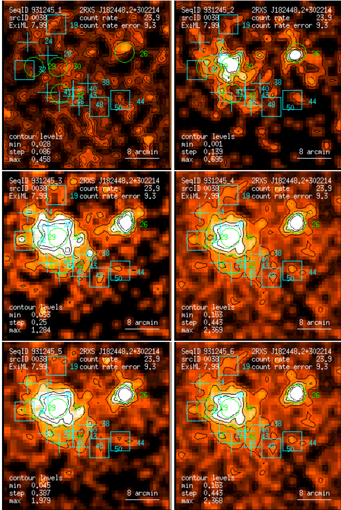
Figure 38: RASS 931245: detection 0038: band rate images, Gaussian filter: (1) PSPC channels 11 – 41, (2) 52 – 90, (3) 91 – 201, (4) 11 – 235, (5) 52 – 201, (6) 11 – 201. Broad band rates in counts/ks. Band rate contour levels in counts/ks/arcmin 2 .
