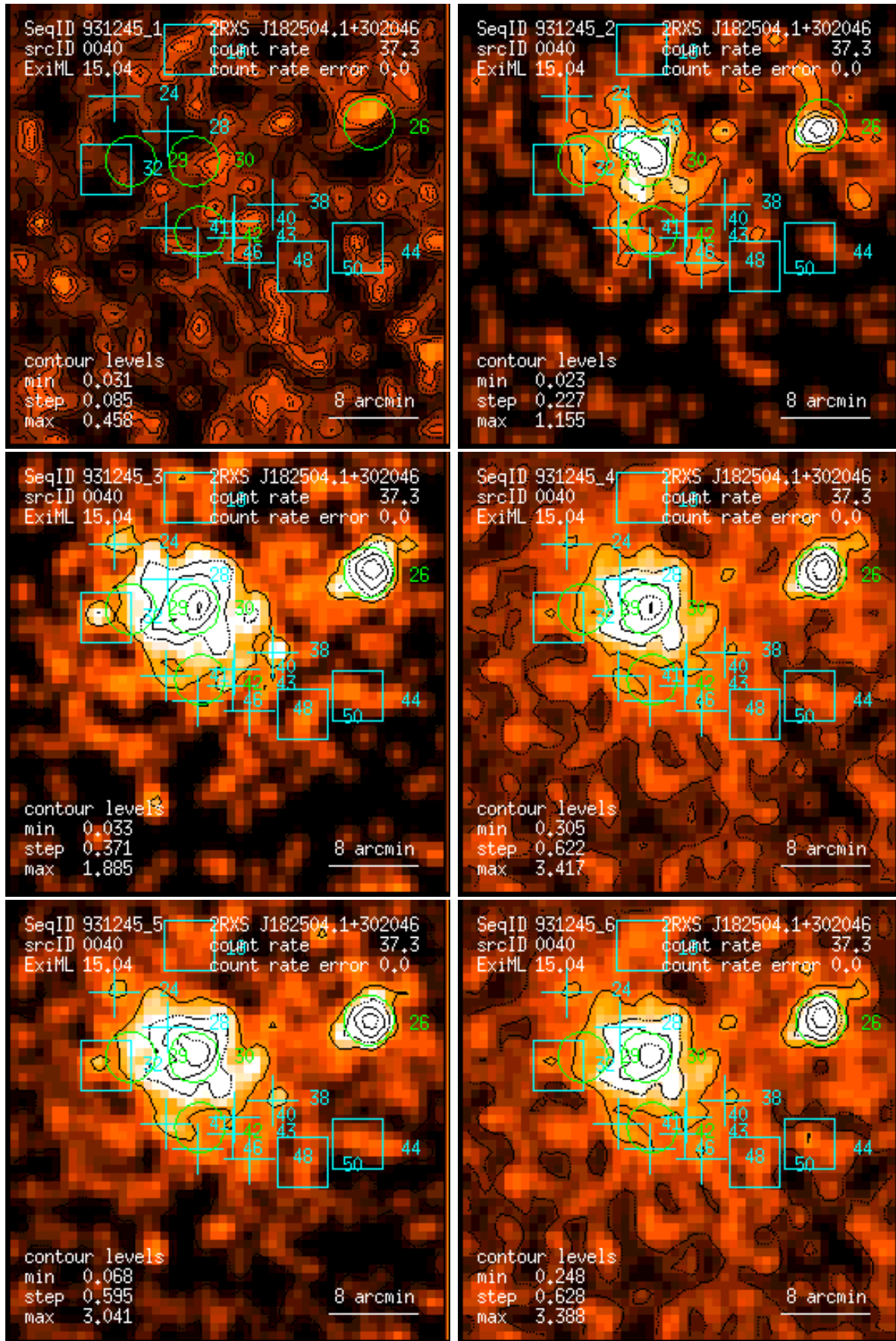
Figure 40: RASS 931245: detection 0040: band rate images, Gaussian filter: (1) PSPC channels 11 – 41, (2) 52 – 90, (3) 91 – 201, (4) 11 – 235, (5) 52 – 201, (6) 11 – 201. Broad band rates in counts/ks. Band rate contour levels in counts/ks/arcmin 2 .
