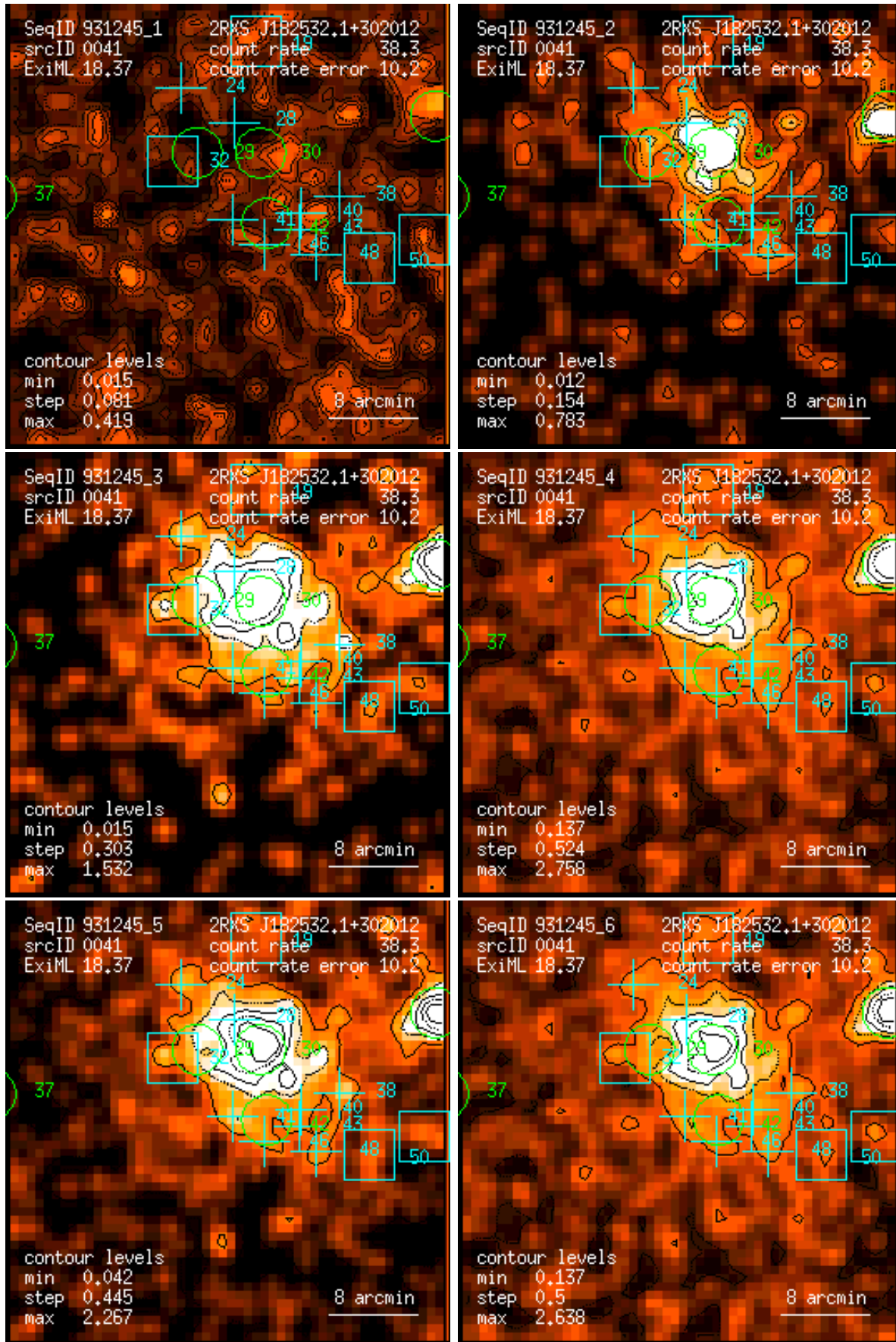
Figure 41: RASS 931245: detection 0041: band rate images, Gaussian filter: (1) PSPC channels 11 – 41, (2) 52 – 90, (3) 91 – 201, (4) 11 – 235, (5) 52 – 201, (6) 11 – 201. Broad band rates in counts/ks. Band rate contour levels in counts/ks/arcmin 2 .
