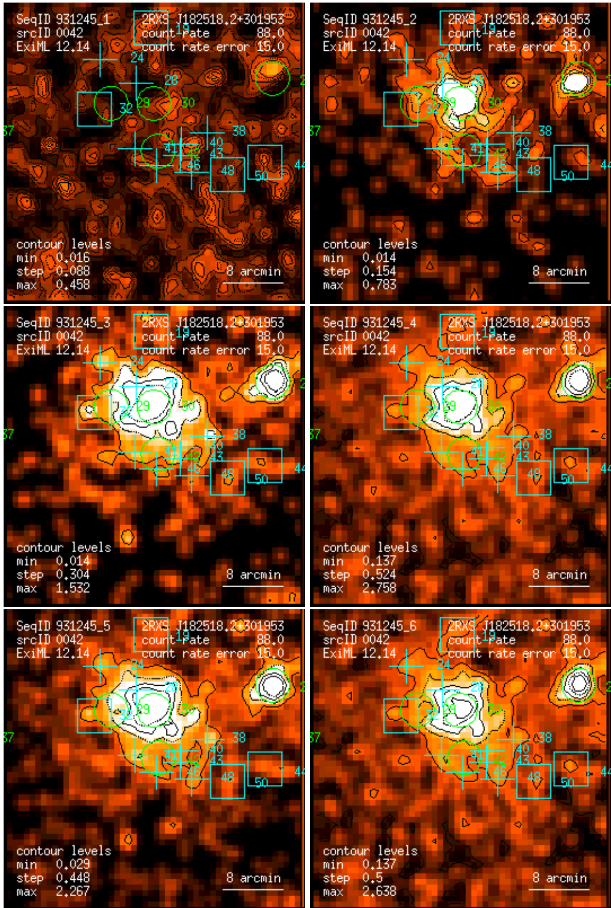
Figure 42: RASS 931245: detection 0042: band rate images, Gaussian filter: (1) PSPC channels 11 – 41, (2) 52 – 90, (3) 91 – 201, (4) 11 – 235, (5) 52 – 201, (6) 11 – 201. Broad band rates in counts/ks. Band rate contour levels in counts/ks/arcmin 2 .
