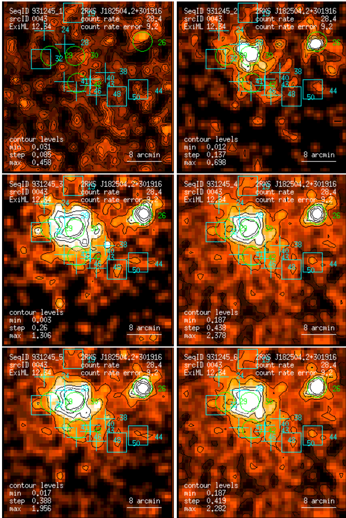
Figure 43: RASS 931245: detection 0043: band rate images, Gaussian filter: (1) PSPC channels 11 – 41, (2) 52 – 90, (3) 91 – 201, (4) 11 – 235, (5) 52 – 201, (6) 11 – 201. Broad band rates in counts/ks. Band rate contour levels in counts/ks/arcmin 2 .
