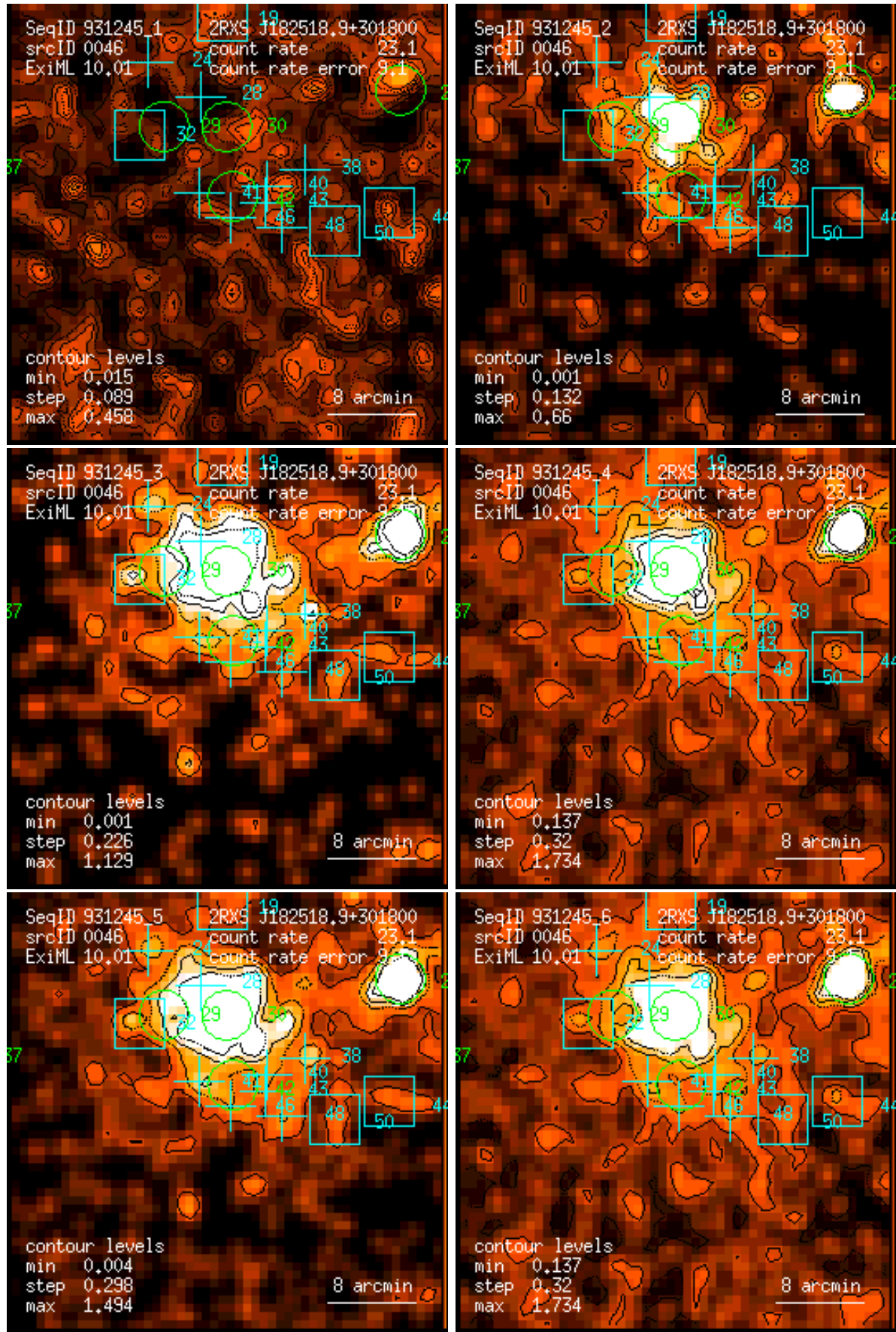
Figure 46: RASS 931245: detection 0046: band rate images, Gaussian filter: (1) PSPC channels 11 – 41, (2) 52 – 90, (3) 91 – 201, (4) 11 – 235, (5) 52 – 201, (6) 11 – 201. Broad band rates in counts/ks. Band rate contour levels in counts/ks/arcmin 2 .
