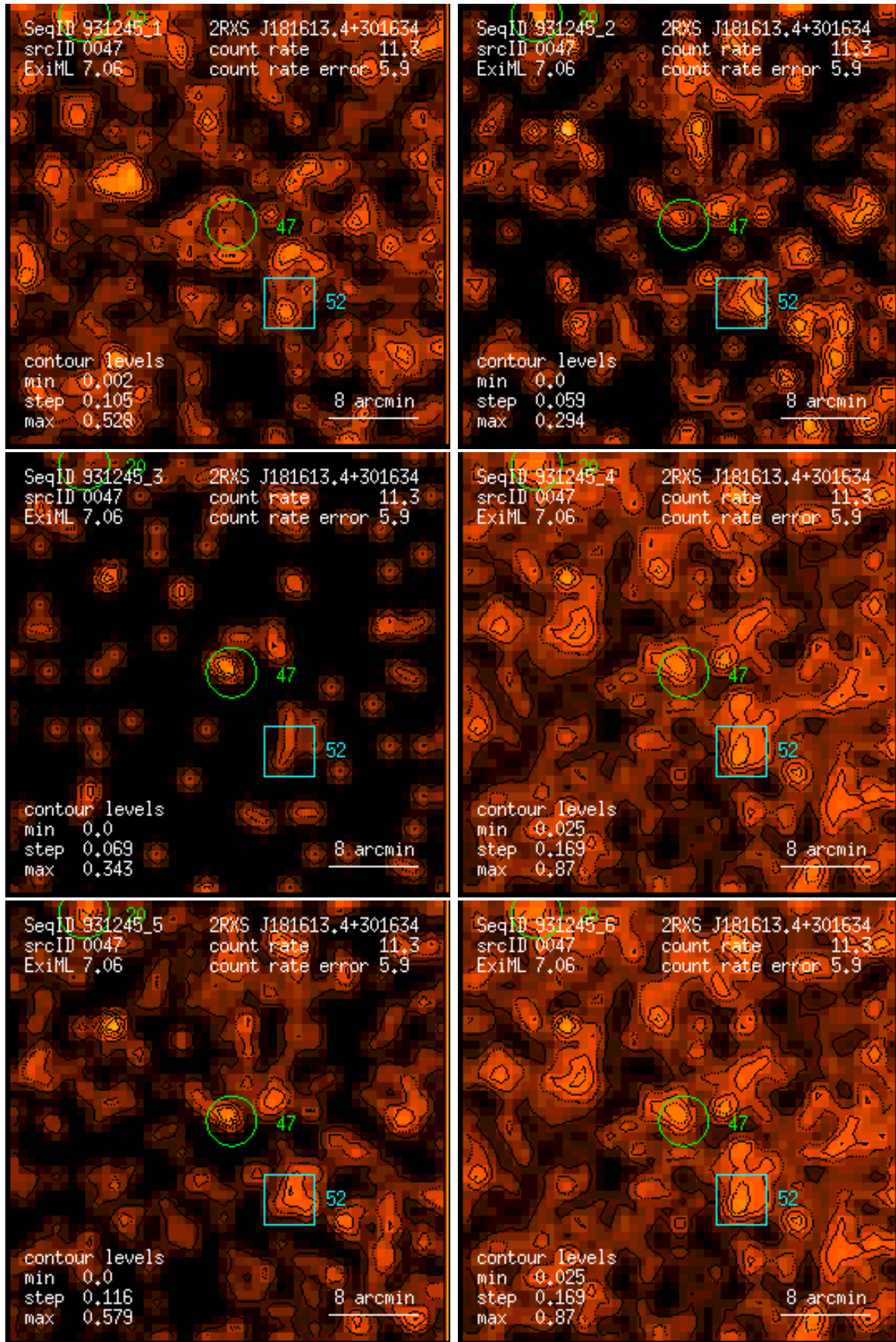
Figure 47: RASS 931245: detection 0047: band rate images, Gaussian filter: (1) PSPC channels 11 – 41, (2) 52 – 90, (3) 91 – 201, (4) 11 – 235, (5) 52 – 201, (6) 11 – 201. Broad band rates in counts/ks. Band rate contour levels in counts/ks/arcmin 2 .
