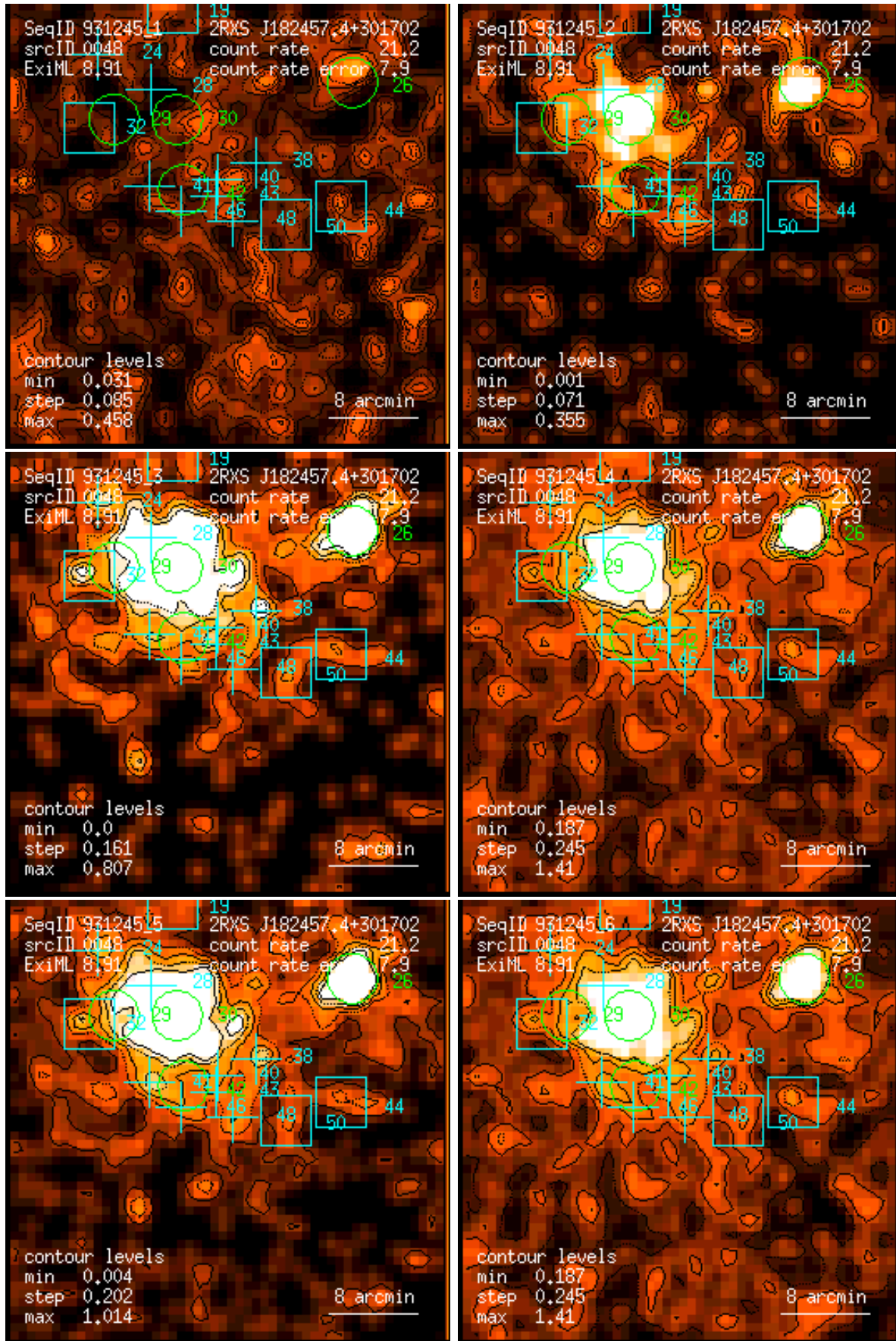
Figure 48: RASS 931245: detection 0048: band rate images, Gaussian filter: (1) PSPC channels 11 – 41, (2) 52 – 90, (3) 91 – 201, (4) 11 – 235, (5) 52 – 201, (6) 11 – 201. Broad band rates in counts/ks. Band rate contour levels in counts/ks/arcmin 2 .
