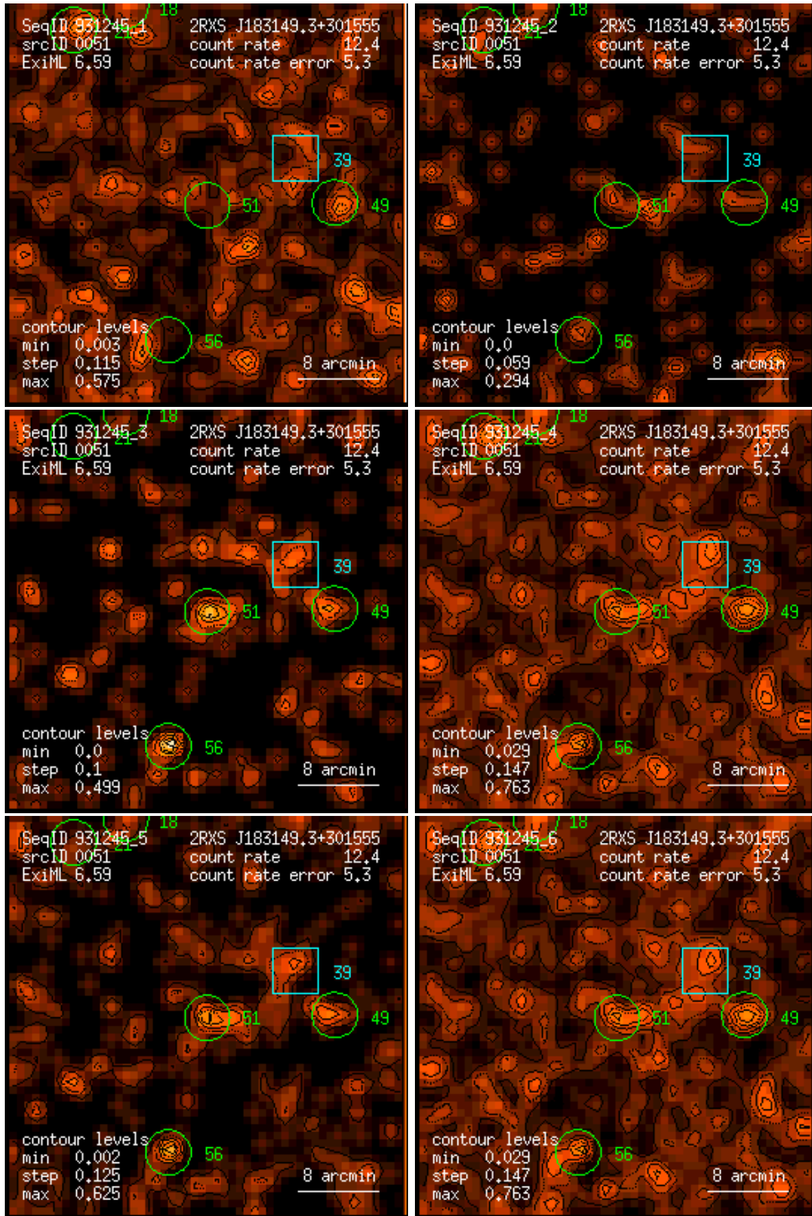
Figure 51: RASS 931245: detection 0051: band rate images, Gaussian filter: (1) PSPC channels 11 – 41, (2) 52 – 90, (3) 91 – 201, (4) 11 – 235, (5) 52 – 201, (6) 11 – 201. Broad band rates in counts/ks. Band rate contour levels in counts/ks/arcmin 2 .
