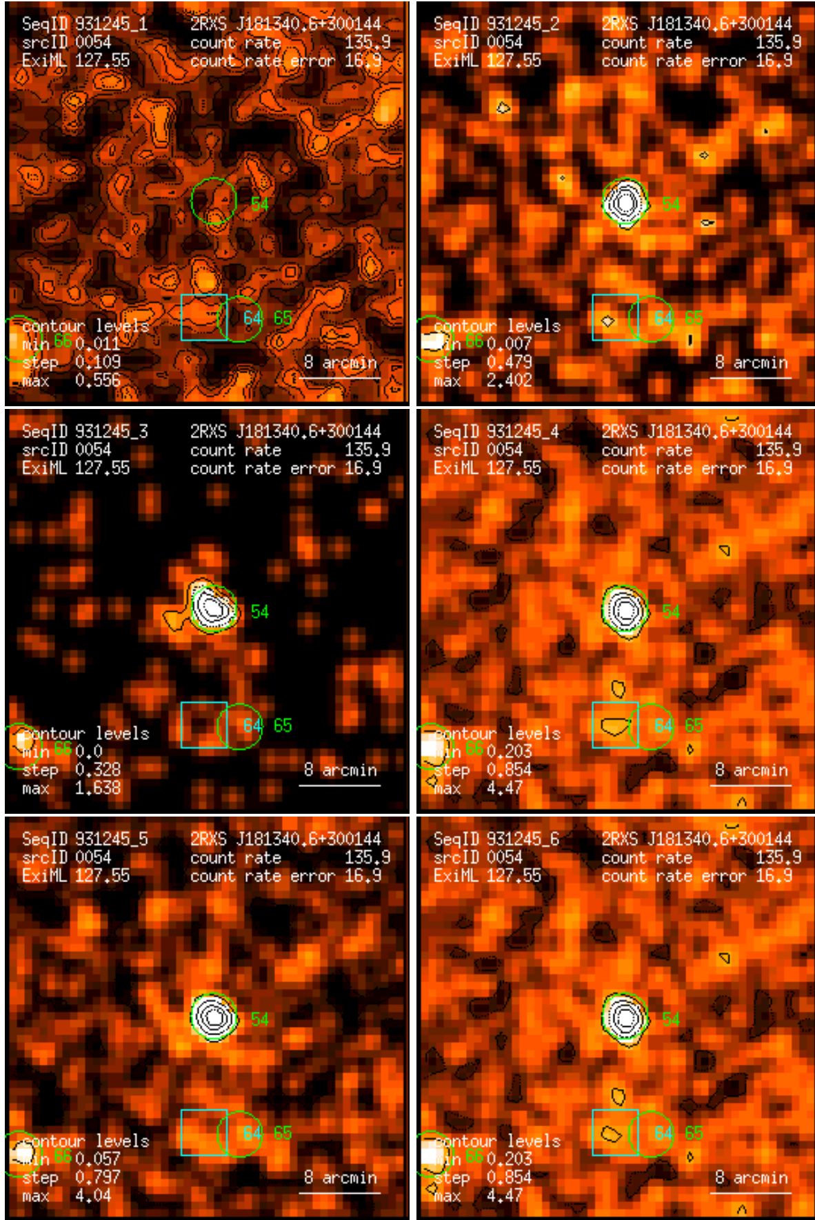
Figure 54: RASS 931245: detection 0054: band rate images, Gaussian filter: (1) PSPC channels 11 – 41, (2) 52 – 90, (3) 91 – 201, (4) 11 – 235, (5) 52 – 201, (6) 11 – 201. Broad band rates in counts/ks. Band rate contour levels in counts/ks/arcmin 2 .
