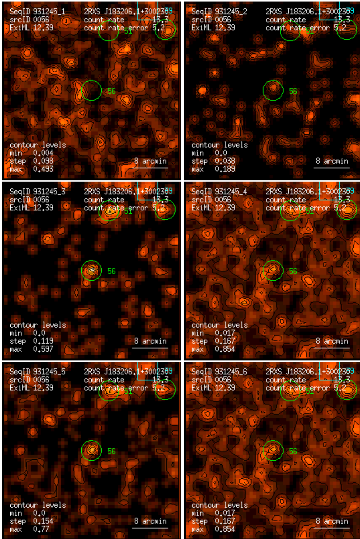
Figure 56: RASS 931245: detection 0056: band rate images, Gaussian filter: (1) PSPC channels 11 – 41, (2) 52 – 90, (3) 91 – 201, (4) 11 – 235, (5) 52 – 201, (6) 11 – 201. Broad band rates in counts/ks. Band rate contour levels in counts/ks/arcmin 2 .
