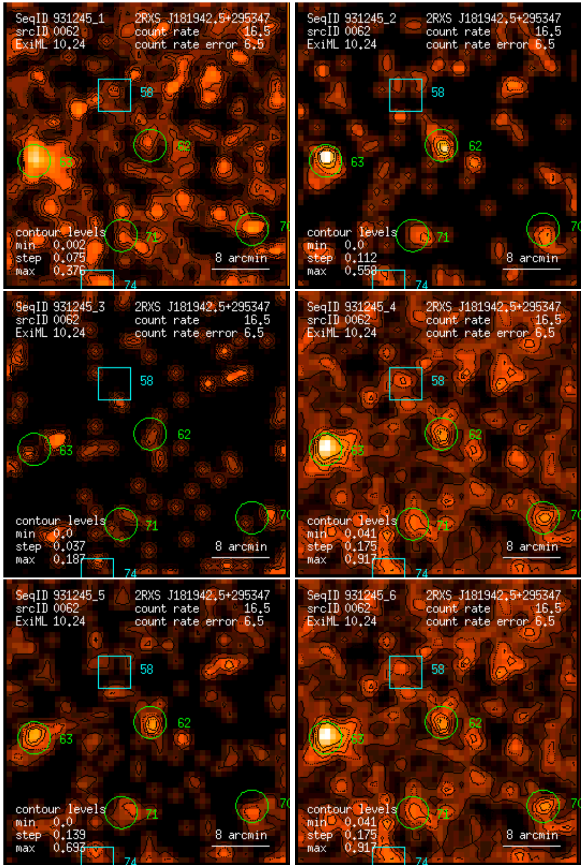
Figure 62: RASS 931245: detection 0062: band rate images, Gaussian filter: (1) PSPC channels 11 – 41, (2) 52 – 90, (3) 91 – 201, (4) 11 – 235, (5) 52 – 201, (6) 11 – 201. Broad band rates in counts/ks. Band rate contour levels in counts/ks/arcmin 2 .
