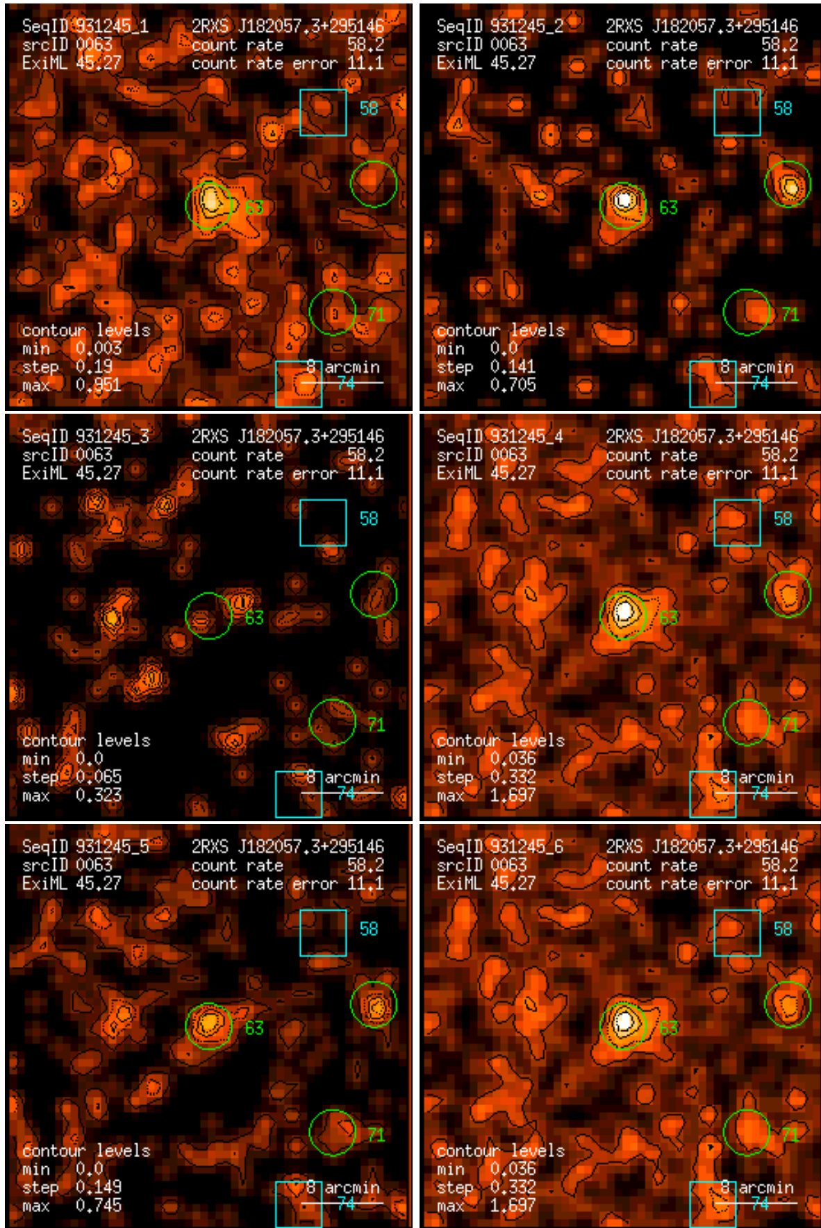
Figure 63: RASS 931245: detection 0063: band rate images, Gaussian filter: (1) PSPC channels 11 – 41, (2) 52 – 90, (3) 91 – 201, (4) 11 – 235, (5) 52 – 201, (6) 11 – 201. Broad band rates in counts/ks. Band rate contour levels in counts/ks/arcmin 2 .
