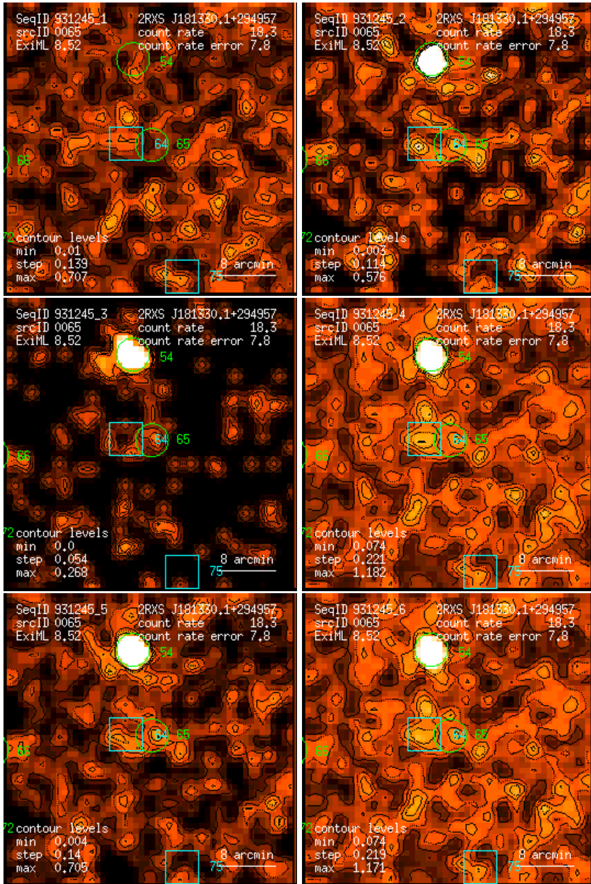
Figure 65: RASS 931245: detection 0065: band rate images, Gaussian filter: (1) PSPC channels 11 – 41, (2) 52 – 90, (3) 91 – 201, (4) 11 – 235, (5) 52 – 201, (6) 11 – 201. Broad band rates in counts/ks. Band rate contour levels in counts/ks/arcmin 2 .
