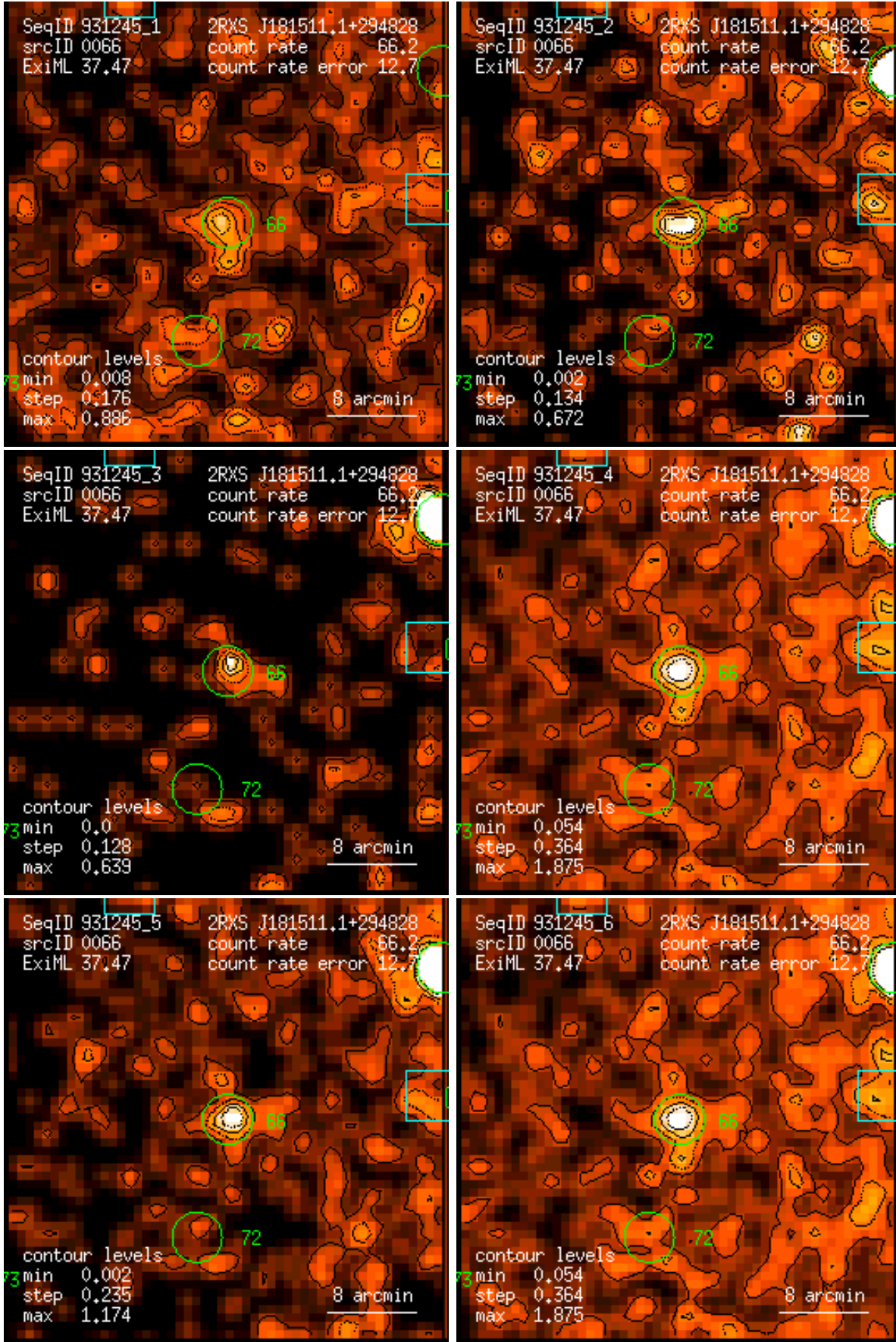
Figure 66: RASS 931245: detection 0066: band rate images, Gaussian filter: (1) PSPC channels 11 – 41, (2) 52 – 90, (3) 91 – 201, (4) 11 – 235, (5) 52 – 201, (6) 11 – 201. Broad band rates in counts/ks. Band rate contour levels in counts/ks/arcmin 2 .
