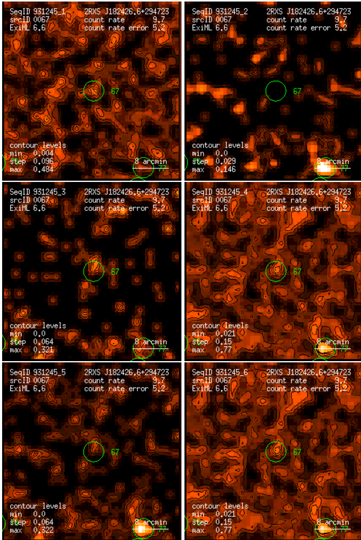
Figure 67: RASS 931245: detection 0067: band rate images, Gaussian filter: (1) PSPC channels 11 – 41, (2) 52 – 90, (3) 91 – 201, (4) 11 – 235, (5) 52 – 201, (6) 11 – 201. Broad band rates in counts/ks. Band rate contour levels in counts/ks/arcmin 2 .
