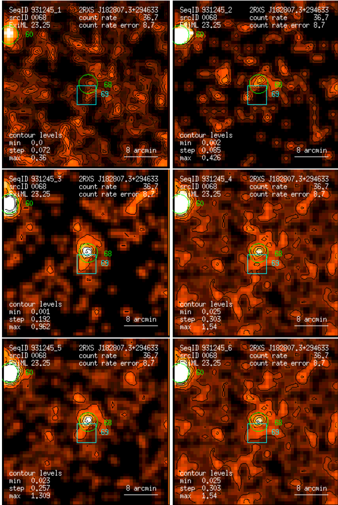
Figure 68: RASS 931245: detection 0068: band rate images, Gaussian filter: (1) PSPC channels 11 – 41, (2) 52 – 90, (3) 91 – 201, (4) 11 – 235, (5) 52 – 201, (6) 11 – 201. Broad band rates in counts/ks. Band rate contour levels in counts/ks/arcmin 2 .
