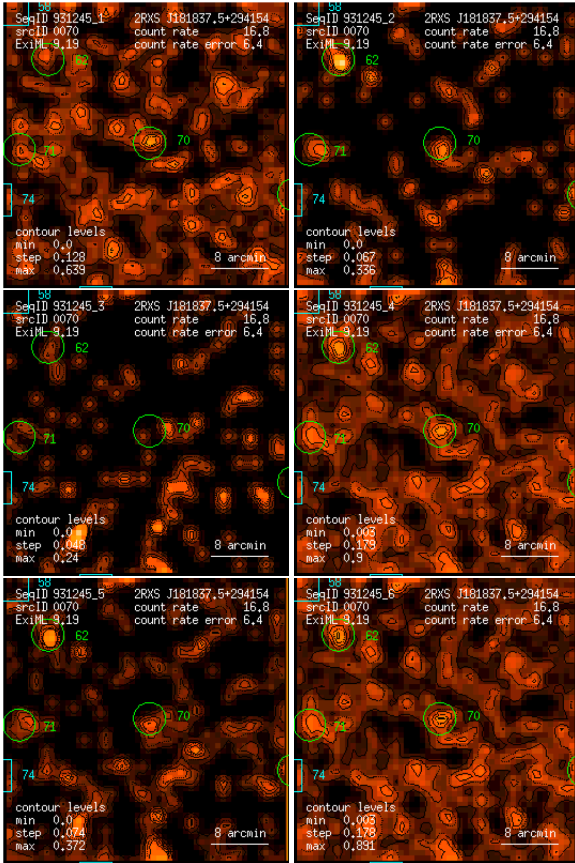
Figure 70: RASS 931245: detection 0070: band rate images, Gaussian filter: (1) PSPC channels 11 – 41, (2) 52 – 90, (3) 91 – 201, (4) 11 – 235, (5) 52 – 201, (6) 11 – 201. Broad band rates in counts/ks. Band rate contour levels in counts/ks/arcmin 2 .
