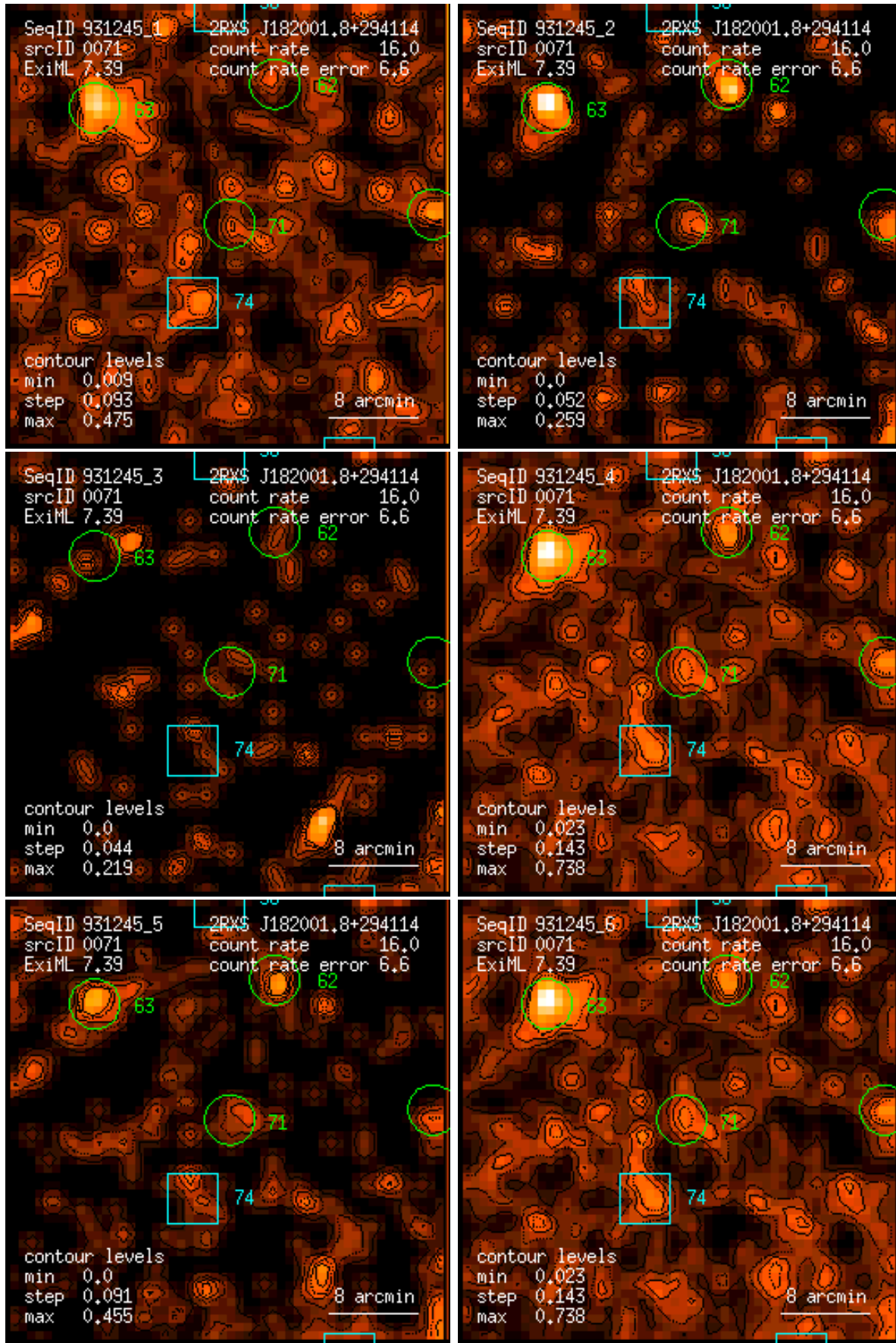
Figure 71: RASS 931245: detection 0071: band rate images, Gaussian filter: (1) PSPC channels 11 – 41, (2) 52 – 90, (3) 91 – 201, (4) 11 – 235, (5) 52 – 201, (6) 11 – 201. Broad band rates in counts/ks. Band rate contour levels in counts/ks/arcmin 2 .
