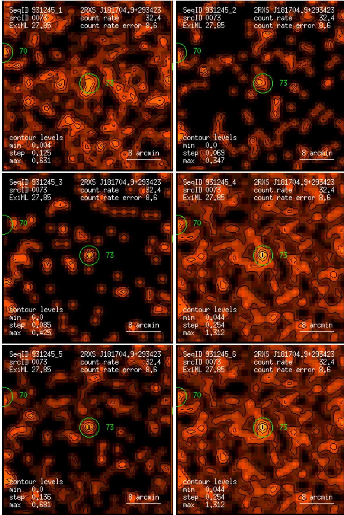
Figure 73: RASS 931245: detection 0073: band rate images, Gaussian filter: (1) PSPC channels 11 – 41, (2) 52 – 90, (3) 91 – 201, (4) 11 – 235, (5) 52 – 201, (6) 11 – 201. Broad band rates in counts/ks. Band rate contour levels in counts/ks/arcmin 2 .
