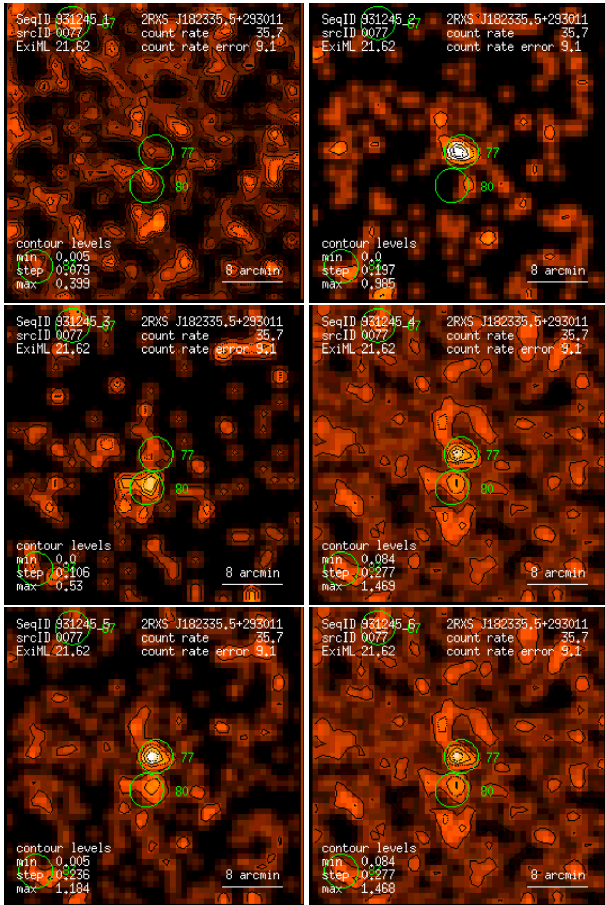
Figure 77: RASS 931245: detection 0077: band rate images, Gaussian filter: (1) PSPC channels 11 – 41, (2) 52 – 90, (3) 91 – 201, (4) 11 – 235, (5) 52 – 201, (6) 11 – 201. Broad band rates in counts/ks. Band rate contour levels in counts/ks/arcmin 2 .
