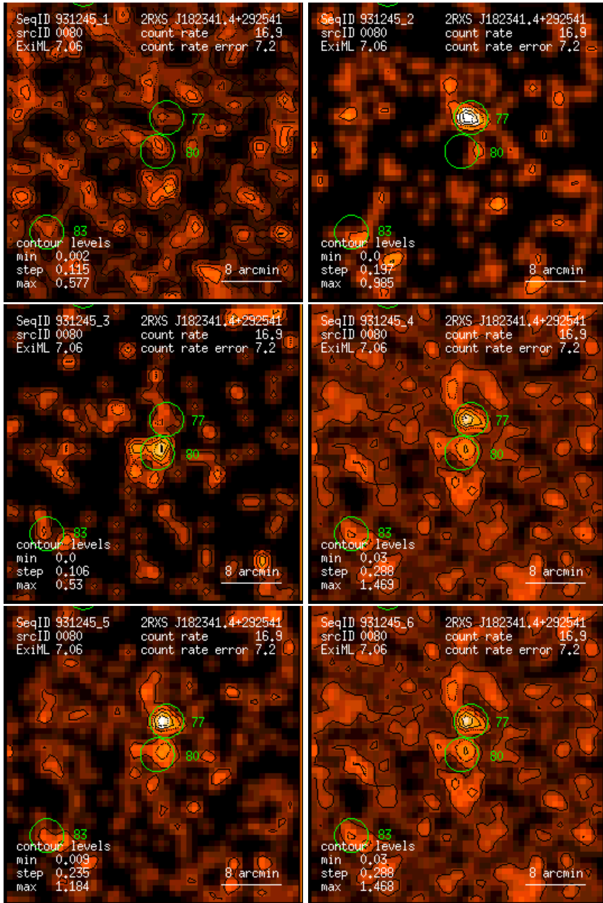
Figure 80: RASS 931245: detection 0080: band rate images, Gaussian filter: (1) PSPC channels 11 – 41, (2) 52 – 90, (3) 91 – 201, (4) 11 – 235, (5) 52 – 201, (6) 11 – 201. Broad band rates in counts/ks. Band rate contour levels in counts/ks/arcmin 2 .
