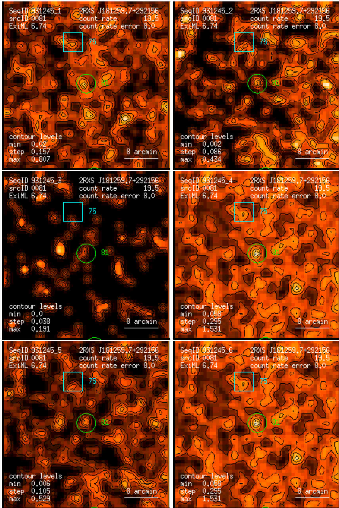
Figure 81: RASS 931245: detection 0081: band rate images, Gaussian filter: (1) PSPC channels 11 – 41, (2) 52 – 90, (3) 91 – 201, (4) 11 – 235, (5) 52 – 201, (6) 11 – 201. Broad band rates in counts/ks. Band rate contour levels in counts/ks/arcmin 2 .
