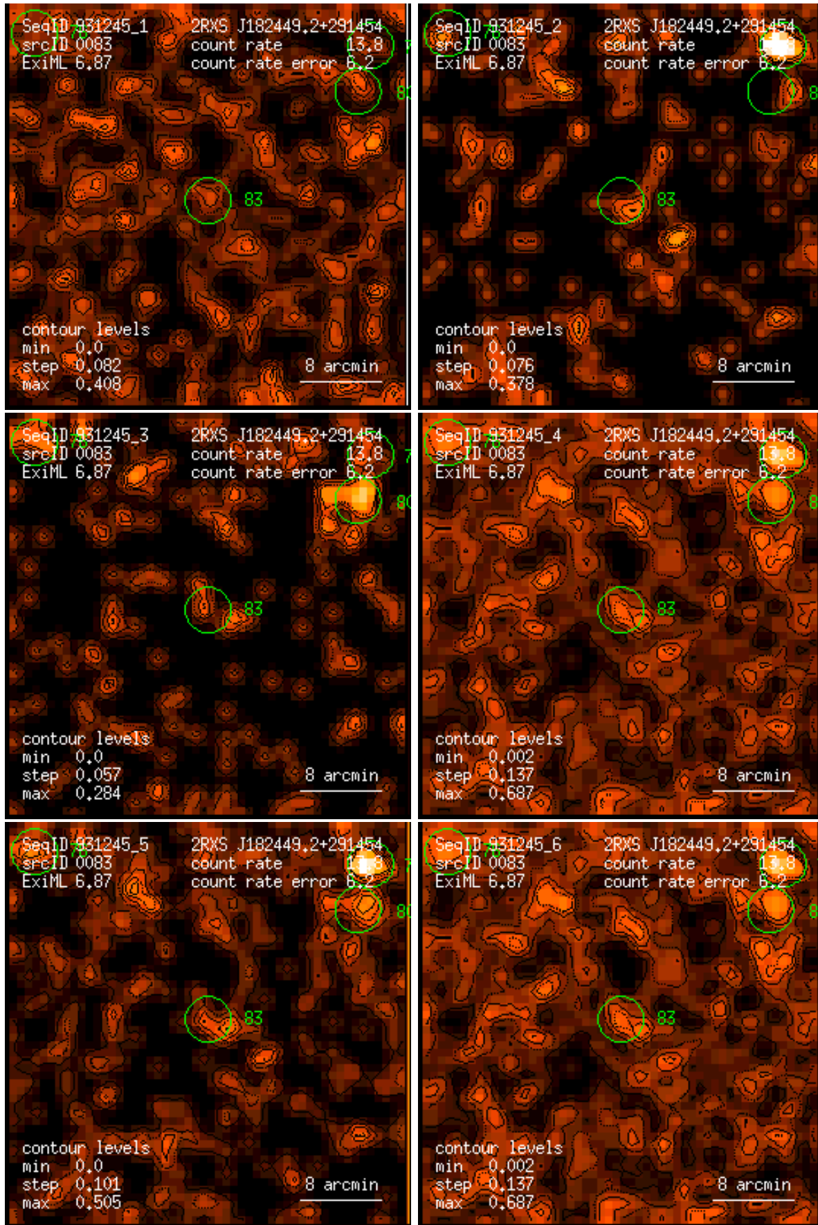
Figure 83: RASS 931245: detection 0083: band rate images, Gaussian filter: (1) PSPC channels 11 – 41, (2) 52 – 90, (3) 91 – 201, (4) 11 – 235, (5) 52 – 201, (6) 11 – 201. Broad band rates in counts/ks. Band rate contour levels in counts/ks/arcmin 2 .
