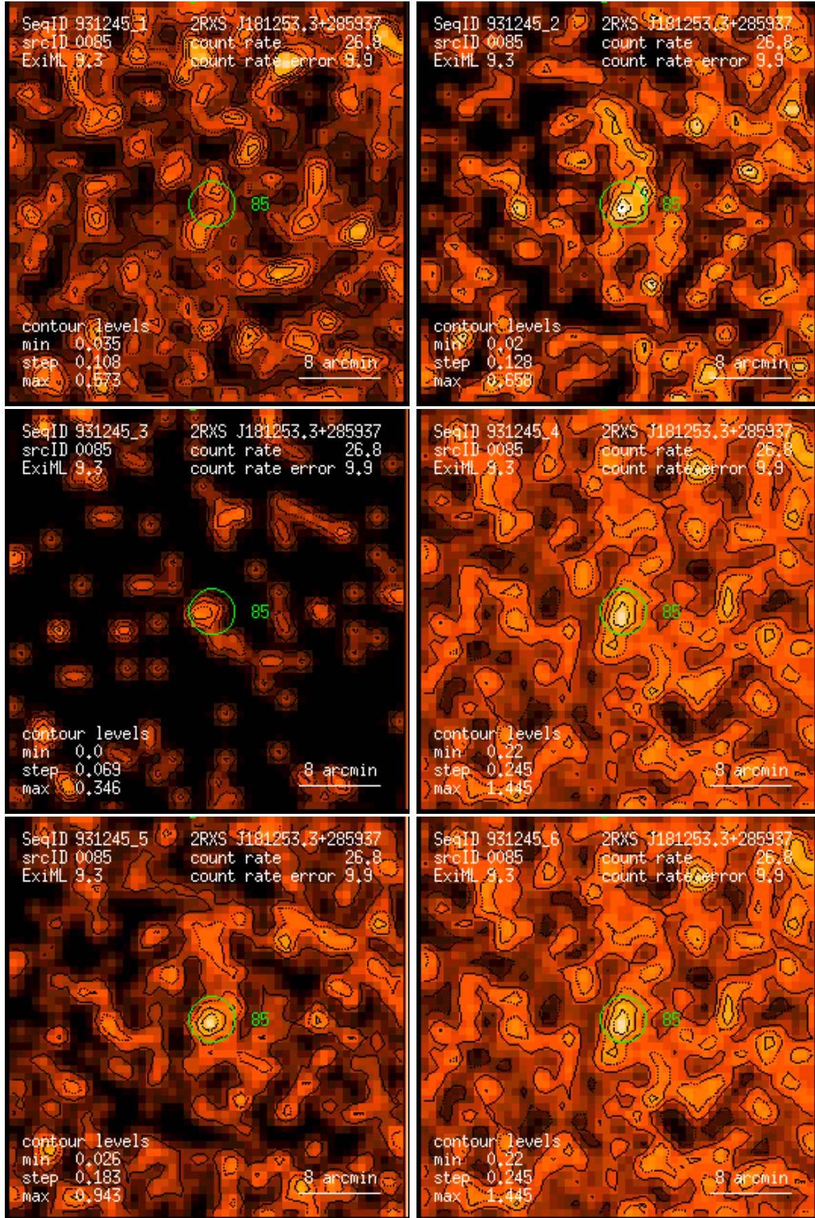
Figure 85: RASS 931245: detection 0085: band rate images, Gaussian filter: (1) PSPC channels 11 – 41, (2) 52 – 90, (3) 91 – 201, (4) 11 – 235, (5) 52 – 201, (6) 11 – 201. Broad band rates in counts/ks. Band rate contour levels in counts/ks/arcmin 2 .
