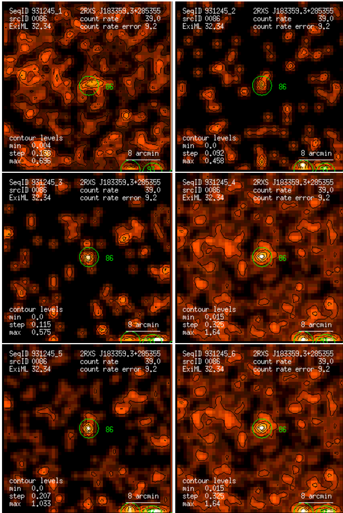
Figure 86: RASS 931245: detection 0086: band rate images, Gaussian filter: (1) PSPC channels 11 – 41, (2) 52 – 90, (3) 91 – 201, (4) 11 – 235, (5) 52 – 201, (6) 11 – 201. Broad band rates in counts/ks. Band rate contour levels in counts/ks/arcmin 2 .
