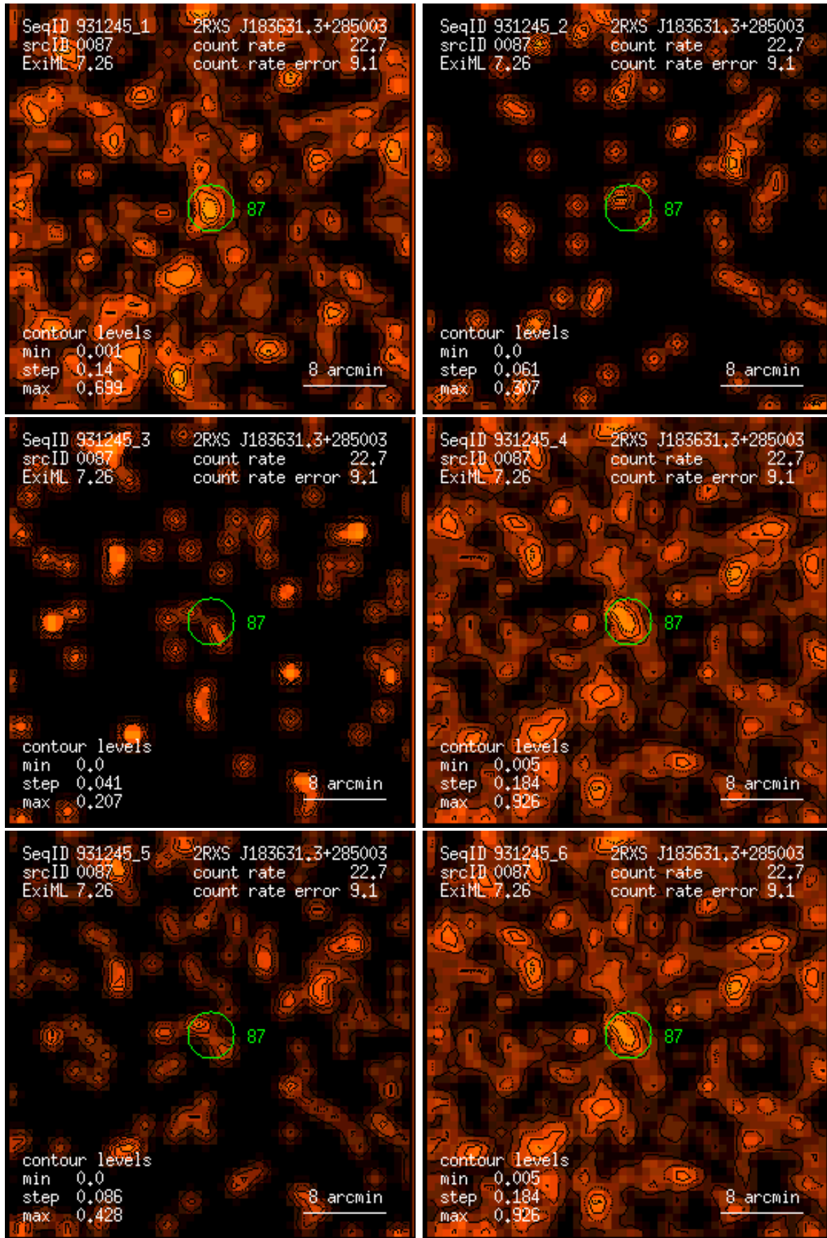
Figure 87: RASS 931245: detection 0087: band rate images, Gaussian filter: (1) PSPC channels 11 – 41, (2) 52 – 90, (3) 91 – 201, (4) 11 – 235, (5) 52 – 201, (6) 11 – 201. Broad band rates in counts/ks. Band rate contour levels in counts/ks/arcmin 2 .
