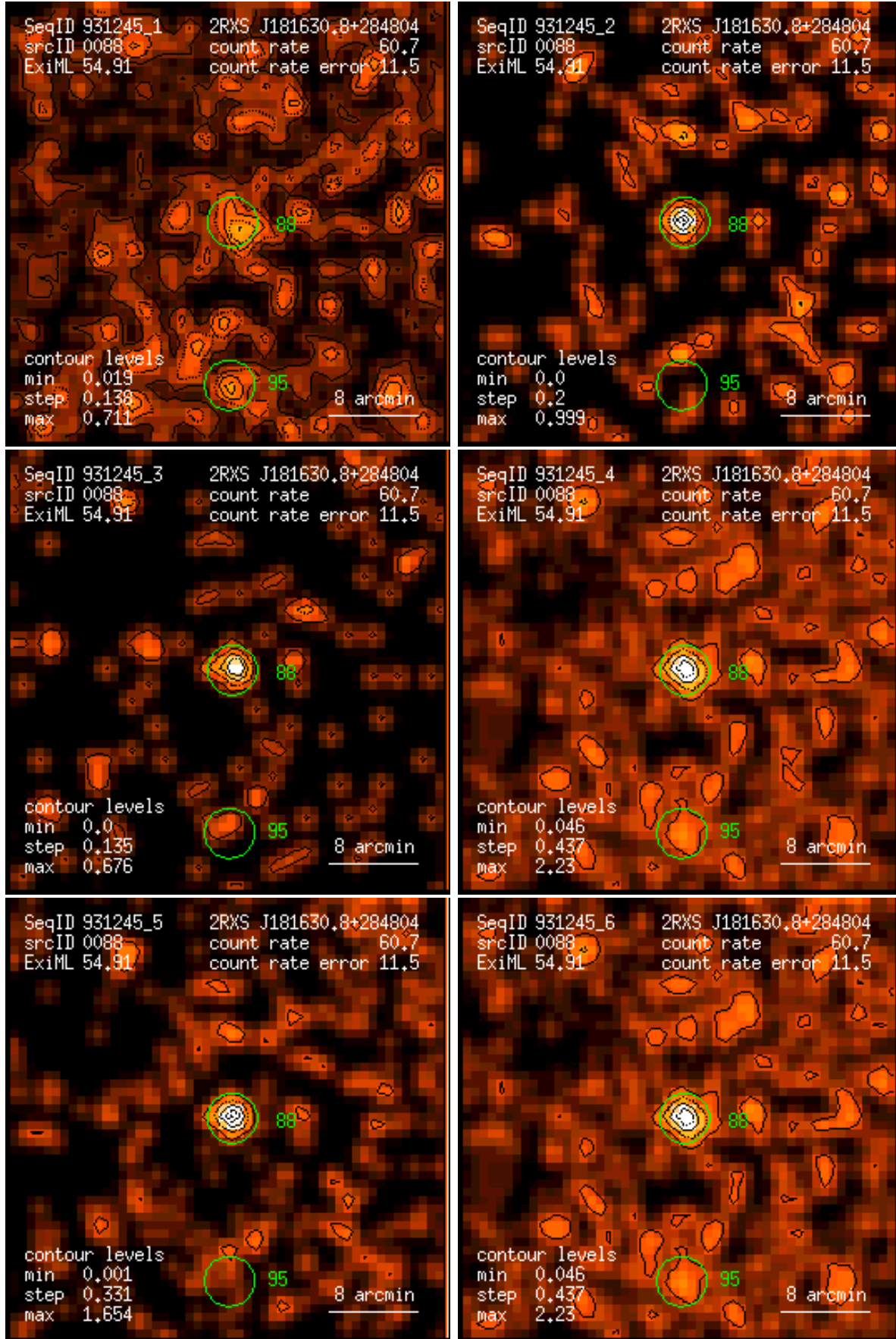
Figure 88: RASS 931245: detection 0088: band rate images, Gaussian filter: (1) PSPC channels 11 – 41, (2) 52 – 90, (3) 91 – 201, (4) 11 – 235, (5) 52 – 201, (6) 11 – 201. Broad band rates in counts/ks. Band rate contour levels in counts/ks/arcmin 2 .
