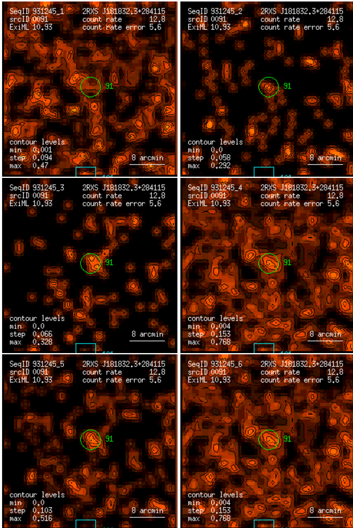
Figure 91: RASS 931245: detection 0091: band rate images, Gaussian filter: (1) PSPC channels 11 – 41, (2) 52 – 90, (3) 91 – 201, (4) 11 – 235, (5) 52 – 201, (6) 11 – 201. Broad band rates in counts/ks. Band rate contour levels in counts/ks/arcmin 2 .
