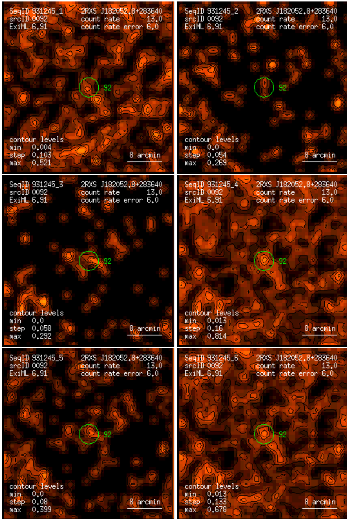
Figure 92: RASS 931245: detection 0092: band rate images, Gaussian filter: (1) PSPC channels 11 – 41, (2) 52 – 90, (3) 91 – 201, (4) 11 – 235, (5) 52 – 201, (6) 11 – 201. Broad band rates in counts/ks. Band rate contour levels in counts/ks/arcmin 2 .
