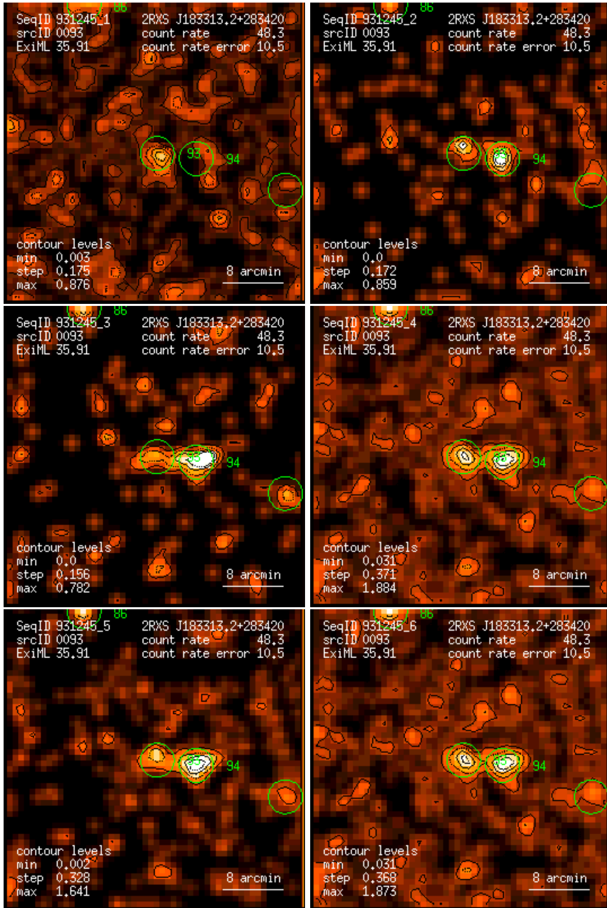
Figure 93: RASS 931245: detection 0093: band rate images, Gaussian filter: (1) PSPC channels 11 – 41, (2) 52 – 90, (3) 91 – 201, (4) 11 – 235, (5) 52 – 201, (6) 11 – 201. Broad band rates in counts/ks. Band rate contour levels in counts/ks/arcmin 2 .
