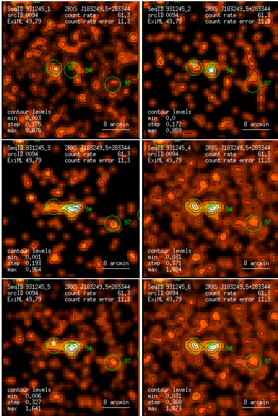
Figure 94: RASS 931245: detection 0094: band rate images, Gaussian filter: (1) PSPC channels 11 – 41, (2) 52 – 90, (3) 91 – 201, (4) 11 – 235, (5) 52 – 201, (6) 11 – 201. Broad band rates in counts/ks. Band rate contour levels in counts/ks/arcmin 2 .
