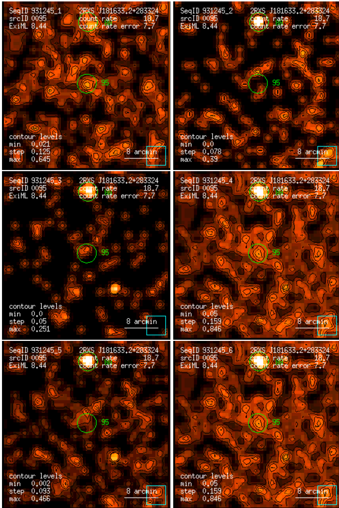
Figure 95: RASS 931245: detection 0095: band rate images, Gaussian filter: (1) PSPC channels 11 – 41, (2) 52 – 90, (3) 91 – 201, (4) 11 – 235, (5) 52 – 201, (6) 11 – 201. Broad band rates in counts/ks. Band rate contour levels in counts/ks/arcmin 2 .
