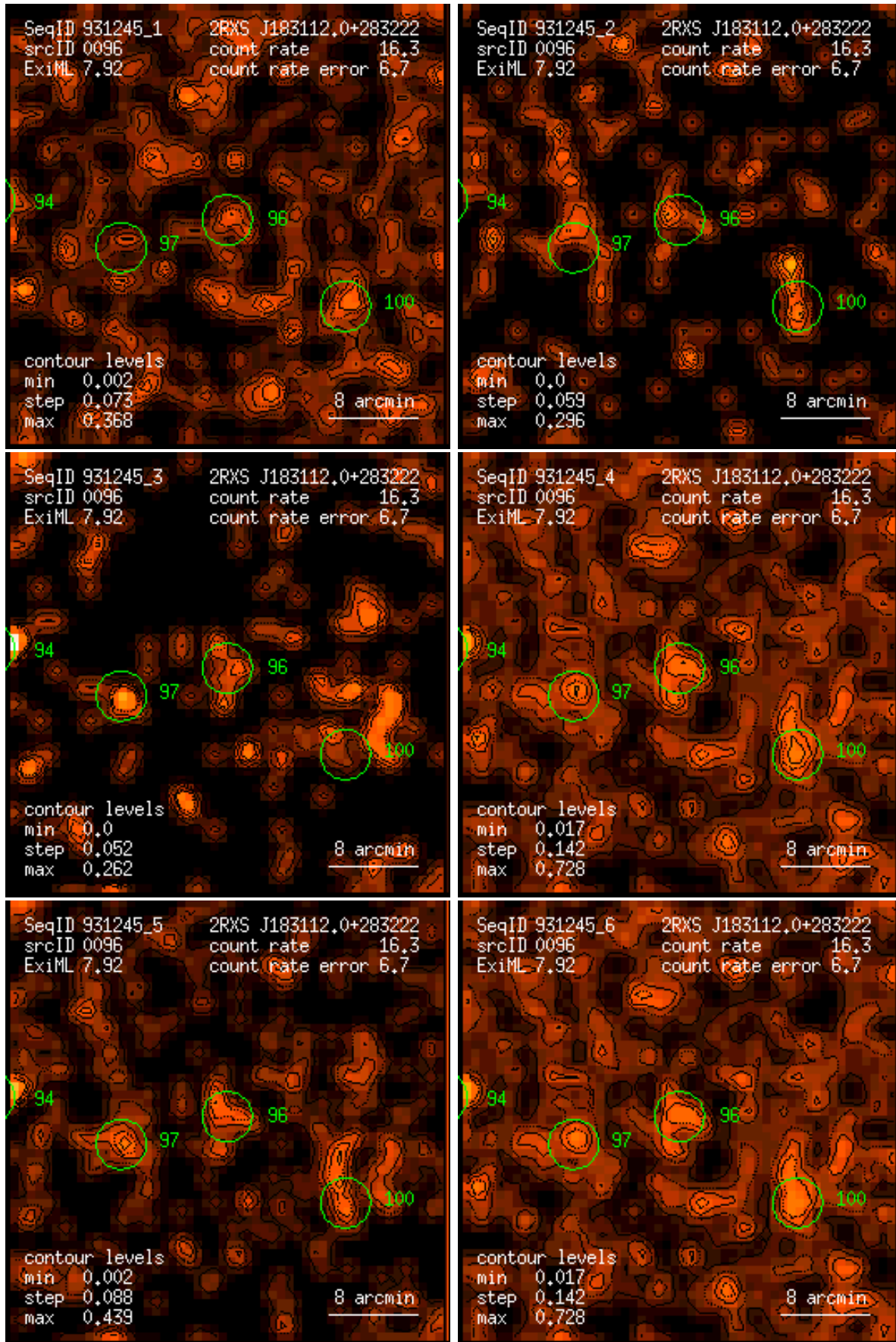
Figure 96: RASS 931245: detection 0096: band rate images, Gaussian filter: (1) PSPC channels 11 – 41, (2) 52 – 90, (3) 91 – 201, (4) 11 – 235, (5) 52 – 201, (6) 11 – 201. Broad band rates in counts/ks. Band rate contour levels in counts/ks/arcmin 2 .
