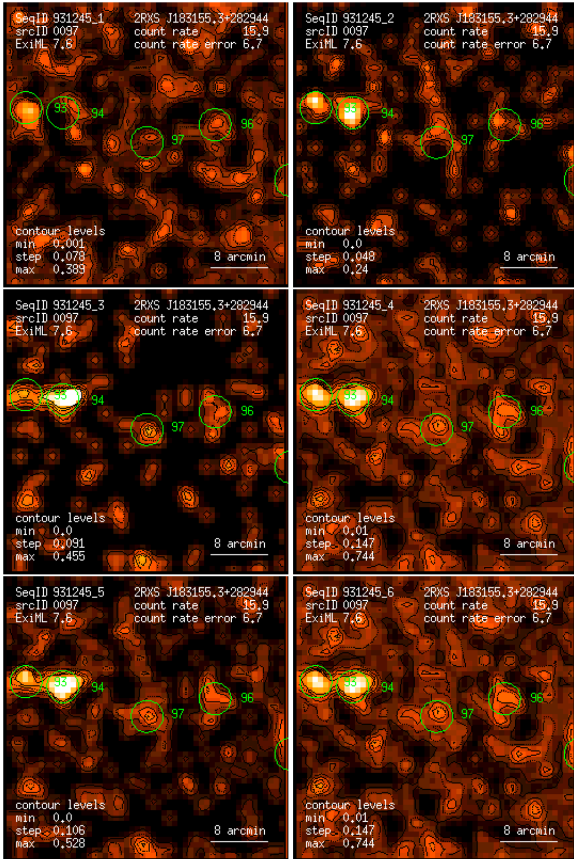
Figure 97: RASS 931245: detection 0097: band rate images, Gaussian filter: (1) PSPC channels 11 – 41, (2) 52 – 90, (3) 91 – 201, (4) 11 – 235, (5) 52 – 201, (6) 11 – 201. Broad band rates in counts/ks. Band rate contour levels in counts/ks/arcmin 2 .
