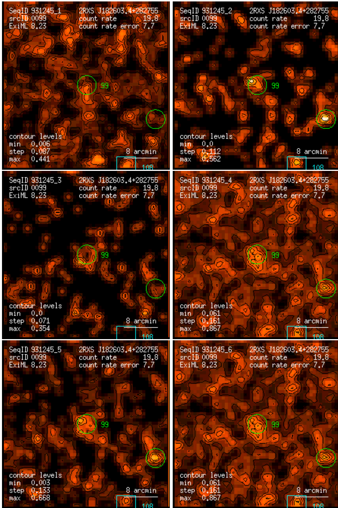
Figure 99: RASS 931245: detection 0099: band rate images, Gaussian filter: (1) PSPC channels 11 – 41, (2) 52 – 90, (3) 91 – 201, (4) 11 – 235, (5) 52 – 201, (6) 11 – 201. Broad band rates in counts/ks. Band rate contour levels in counts/ks/arcmin 2 .
