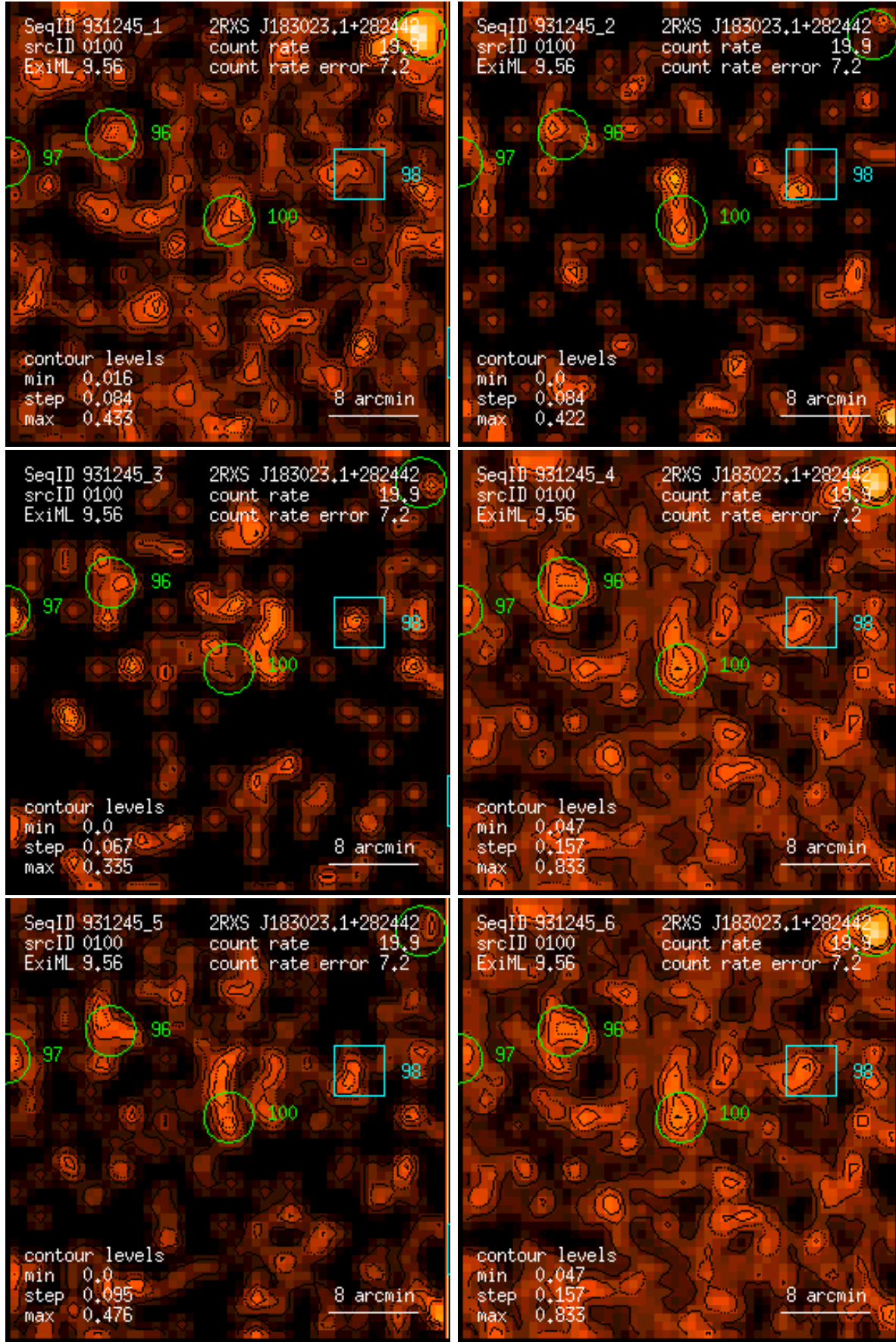
Figure 100: RASS 931245: detection 0100: band rate images, Gaussian filter: (1) PSPC channels 11 – 41, (2) 52 – 90, (3) 91 – 201, (4) 11 – 235, (5) 52 – 201, (6) 11 – 201. Broad band rates in counts/ks. Band rate contour levels in counts/ks/arcmin 2 .
