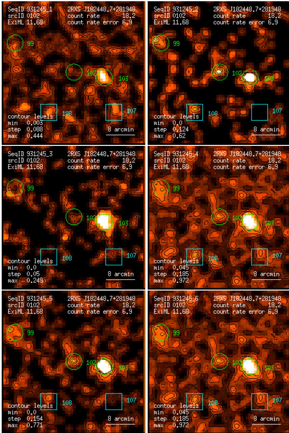
Figure 102: RASS 931245: detection 0102: band rate images, Gaussian filter: (1) PSPC channels 11 – 41, (2) 52 – 90, (3) 91 – 201, (4) 11 – 235, (5) 52 – 201, (6) 11 – 201. Broad band rates in counts/ks. Band rate contour levels in counts/ks/arcmin 2 .
