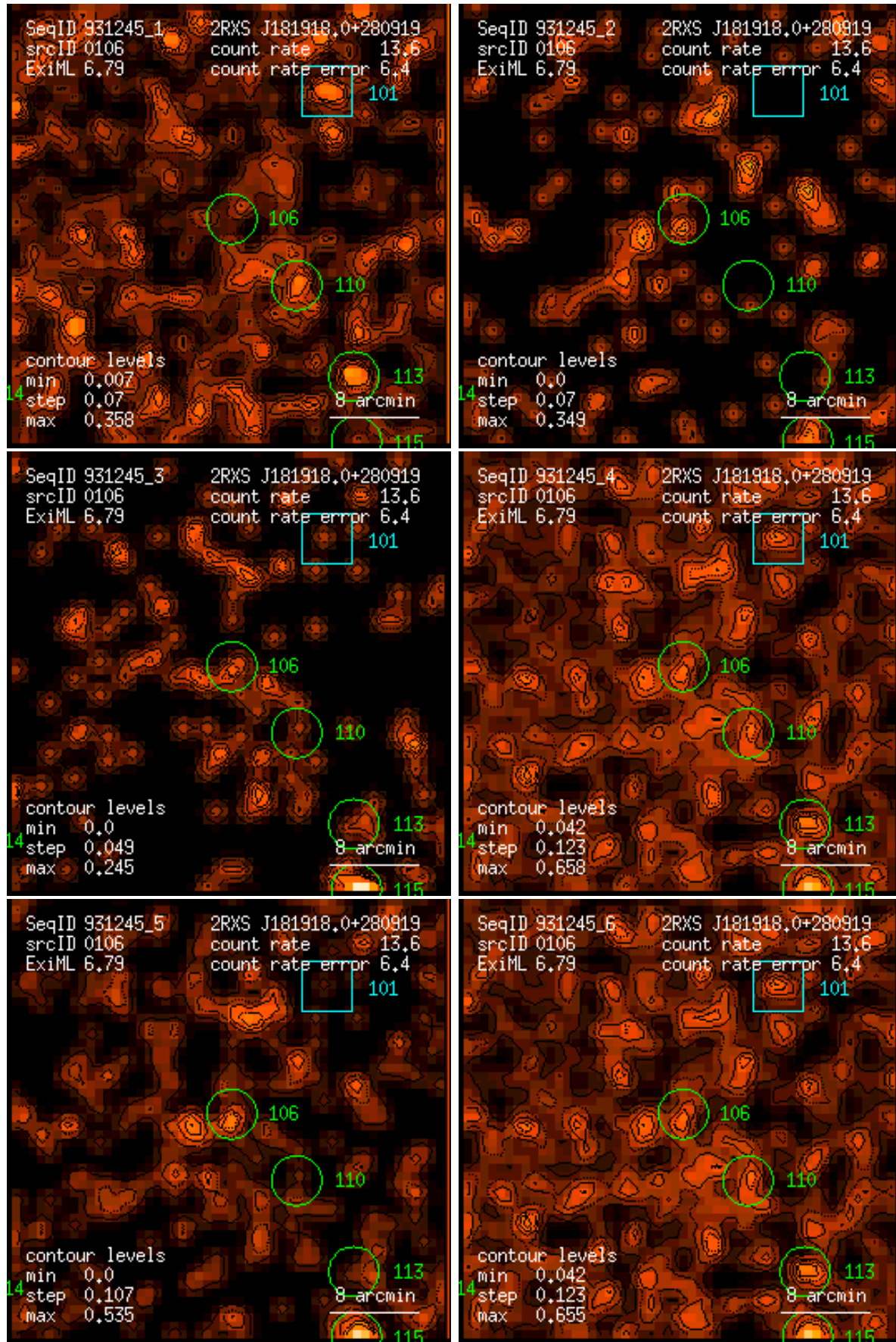
Figure 106: RASS 931245: detection 0106: band rate images, Gaussian filter: (1) PSPC channels 11 – 41, (2) 52 – 90, (3) 91 – 201, (4) 11 – 235, (5) 52 – 201, (6) 11 – 201. Broad band rates in counts/ks. Band rate contour levels in counts/ks/arcmin 2 .
