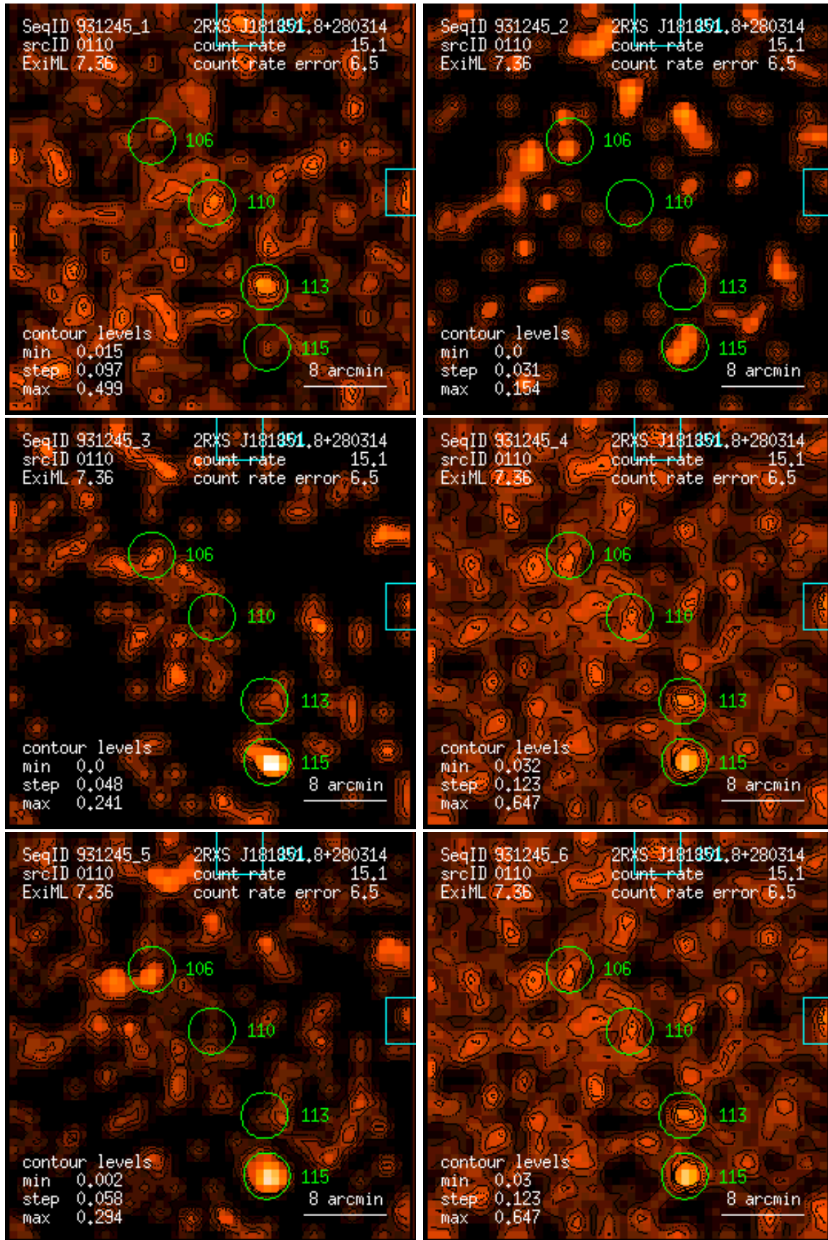
Figure 110: RASS 931245: detection 0110: band rate images, Gaussian filter: (1) PSPC channels 11 – 41, (2) 52 – 90, (3) 91 – 201, (4) 11 – 235, (5) 52 – 201, (6) 11 – 201. Broad band rates in counts/ks. Band rate contour levels in counts/ks/arcmin 2 .
