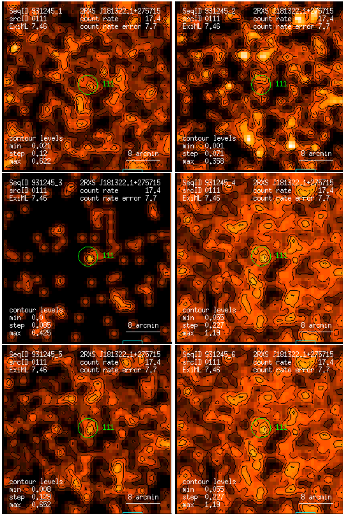
Figure 111: RASS 931245: detection 0111: band rate images, Gaussian filter: (1) PSPC channels 11 – 41, (2) 52 – 90, (3) 91 – 201, (4) 11 – 235, (5) 52 – 201, (6) 11 – 201. Broad band rates in counts/ks. Band rate contour levels in counts/ks/arcmin 2 .
