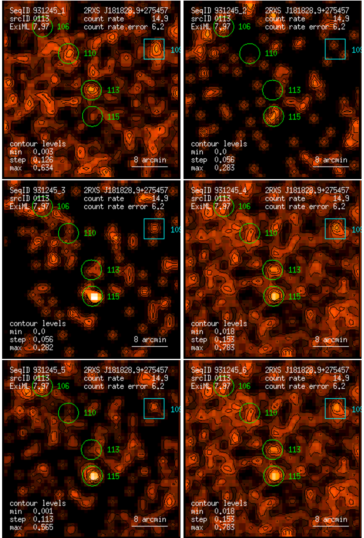
Figure 113: RASS 931245: detection 0113: band rate images, Gaussian filter: (1) PSPC channels 11 – 41, (2) 52 – 90, (3) 91 – 201, (4) 11 – 235, (5) 52 – 201, (6) 11 – 201. Broad band rates in counts/ks. Band rate contour levels in counts/ks/arcmin 2 .
