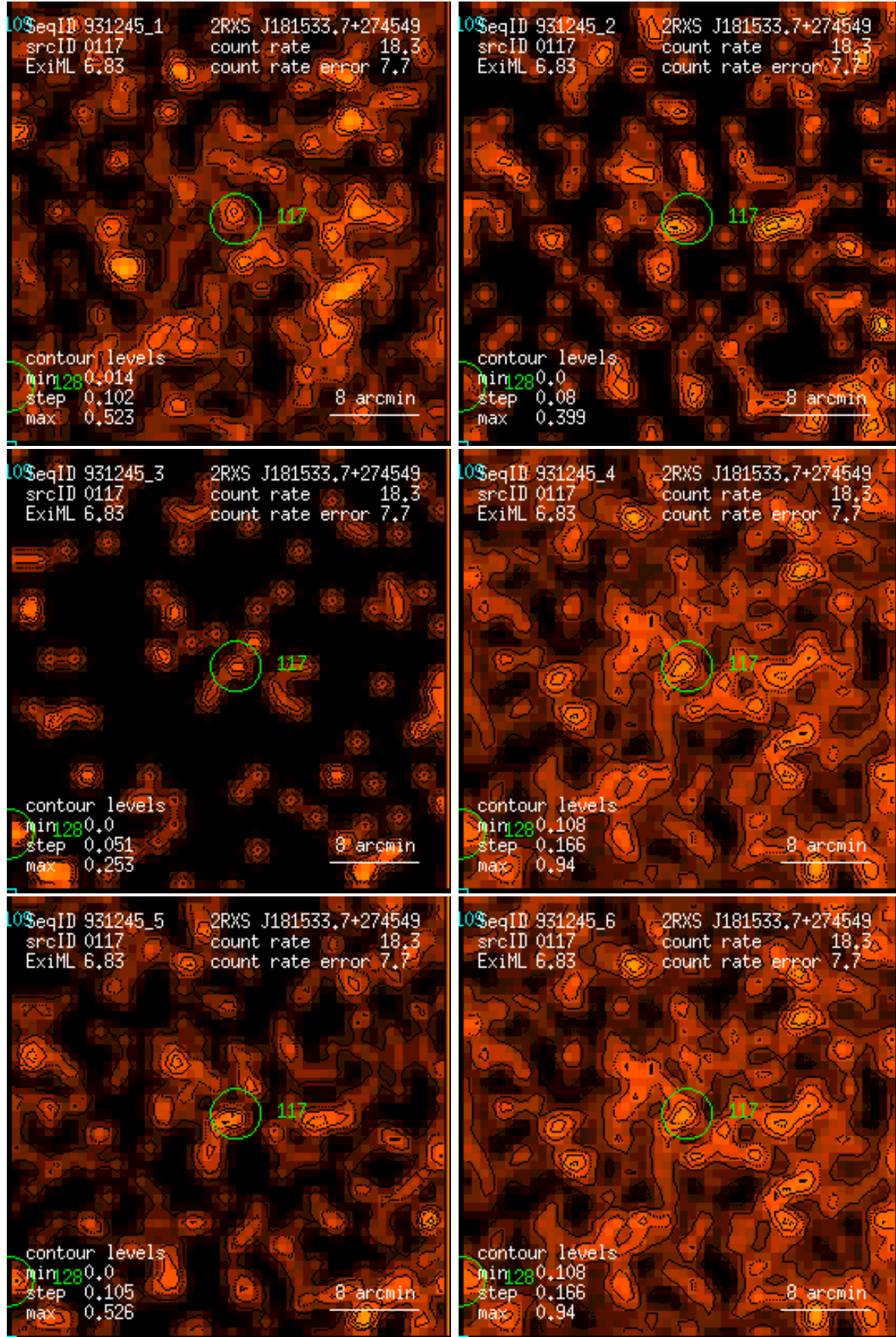
Figure 117: RASS 931245: detection 0117: band rate images, Gaussian filter: (1) PSPC channels 11 – 41, (2) 52 – 90, (3) 91 – 201, (4) 11 – 235, (5) 52 – 201, (6) 11 – 201. Broad band rates in counts/ks. Band rate contour levels in counts/ks/arcmin 2 .
