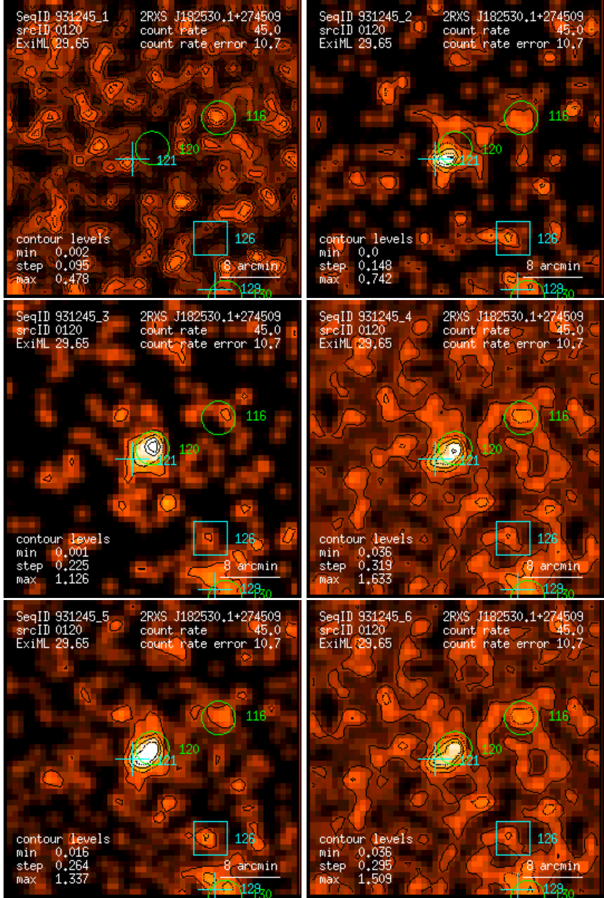
Figure 120: RASS 931245: detection 0120: band rate images, Gaussian filter: (1) PSPC channels 11 – 41, (2) 52 – 90, (3) 91 – 201, (4) 11 – 235, (5) 52 – 201, (6) 11 – 201. Broad band rates in counts/ks. Band rate contour levels in counts/ks/arcmin 2 .
