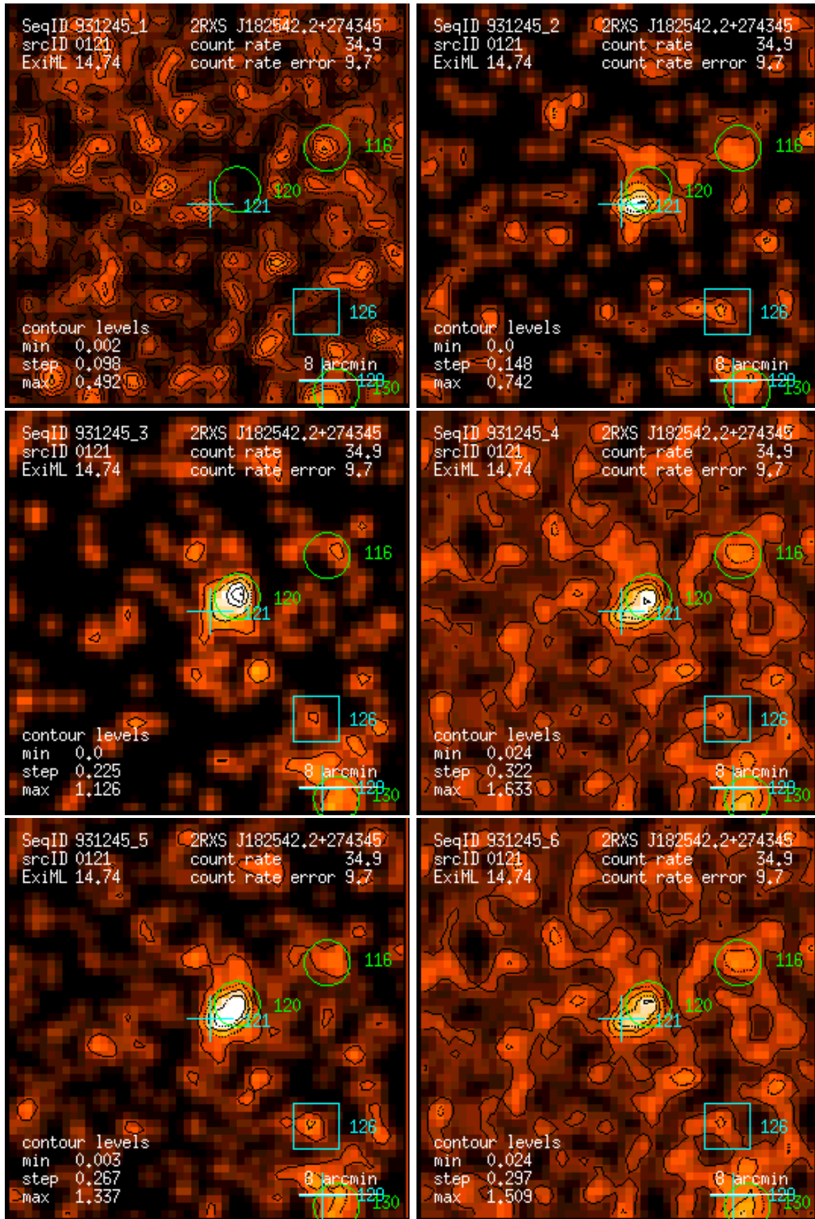
Figure 121: RASS 931245: detection 0121: band rate images, Gaussian filter: (1) PSPC channels 11 – 41, (2) 52 – 90, (3) 91 – 201, (4) 11 – 235, (5) 52 – 201, (6) 11 – 201. Broad band rates in counts/ks. Band rate contour levels in counts/ks/arcmin 2 .
