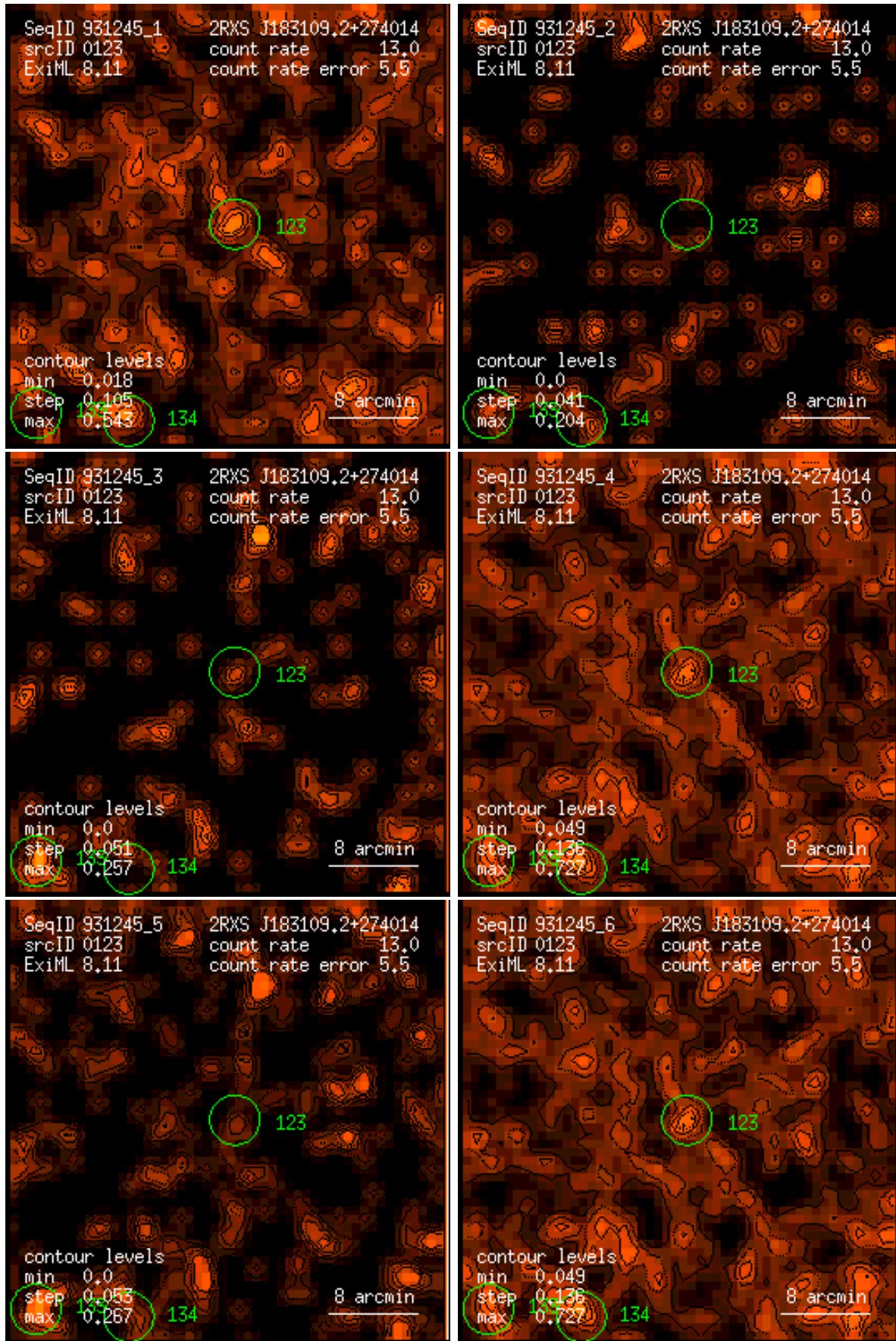
Figure 123: RASS 931245: detection 0123: band rate images, Gaussian filter: (1) PSPC channels 11 – 41, (2) 52 – 90, (3) 91 – 201, (4) 11 – 235, (5) 52 – 201, (6) 11 – 201. Broad band rates in counts/ks. Band rate contour levels in counts/ks/arcmin 2 .
