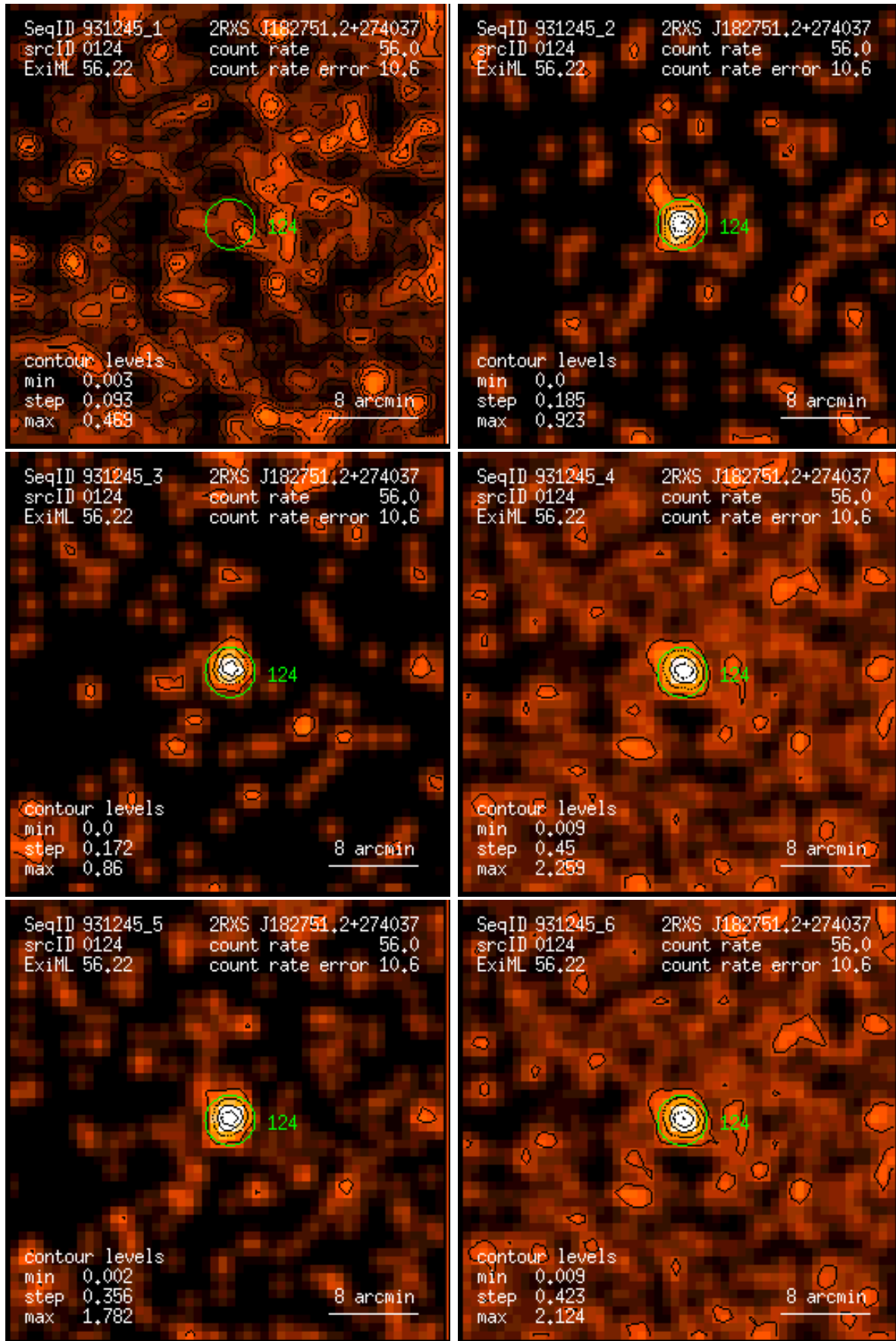
Figure 124: RASS 931245: detection 0124: band rate images, Gaussian filter: (1) PSPC channels 11 – 41, (2) 52 – 90, (3) 91 – 201, (4) 11 – 235, (5) 52 – 201, (6) 11 – 201. Broad band rates in counts/ks. Band rate contour levels in counts/ks/arcmin 2 .
