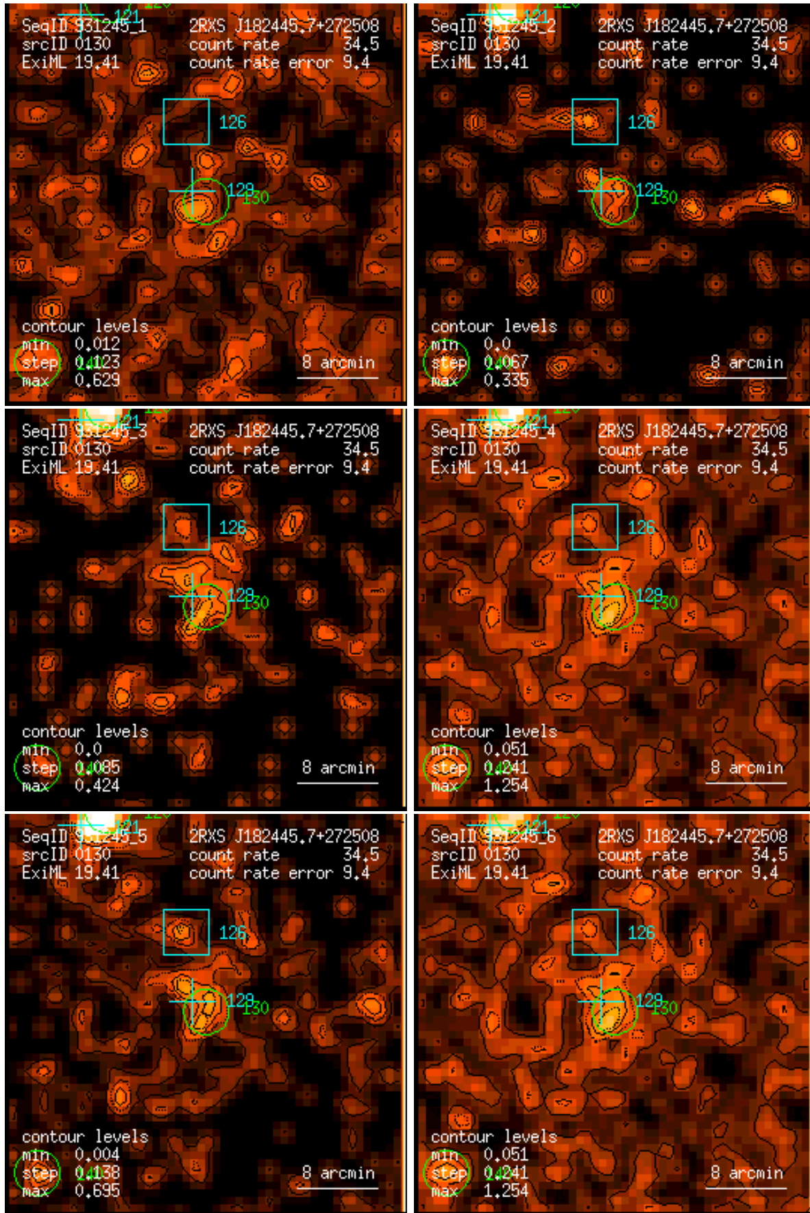
Figure 130: RASS 931245: detection 0130: band rate images, Gaussian filter: (1) PSPC channels 11 – 41, (2) 52 – 90, (3) 91 – 201, (4) 11 – 235, (5) 52 – 201, (6) 11 – 201. Broad band rates in counts/ks. Band rate contour levels in counts/ks/arcmin 2 .
