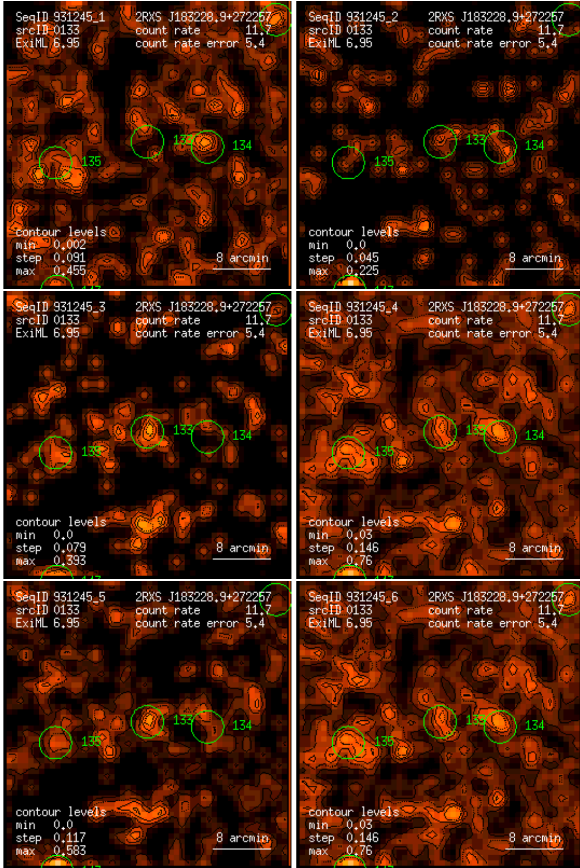
Figure 133: RASS 931245: detection 0133: band rate images, Gaussian filter: (1) PSPC channels 11 – 41, (2) 52 – 90, (3) 91 – 201, (4) 11 – 235, (5) 52 – 201, (6) 11 – 201. Broad band rates in counts/ks. Band rate contour levels in counts/ks/arcmin 2 .
